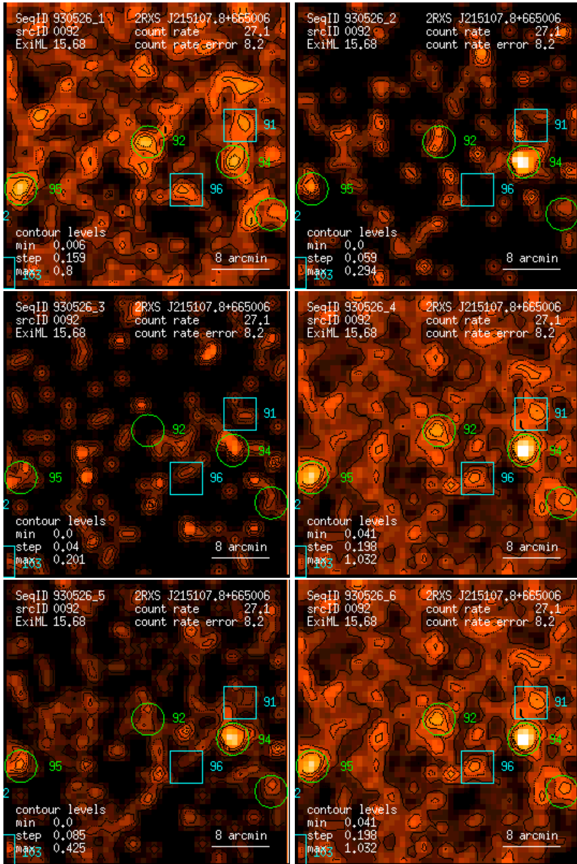
Figure 92: RASS 930526: detection 0092: band rate images, Gaussian filter: (1) PSPC channels 11 – 41, (2) 52 – 90, (3) 91 – 201, (4) 11 – 235, (5) 52 – 201, (6) 11 – 201. Broad band rates in counts/ks. Band rate contour levels in counts/ks/arcmin 2 .
