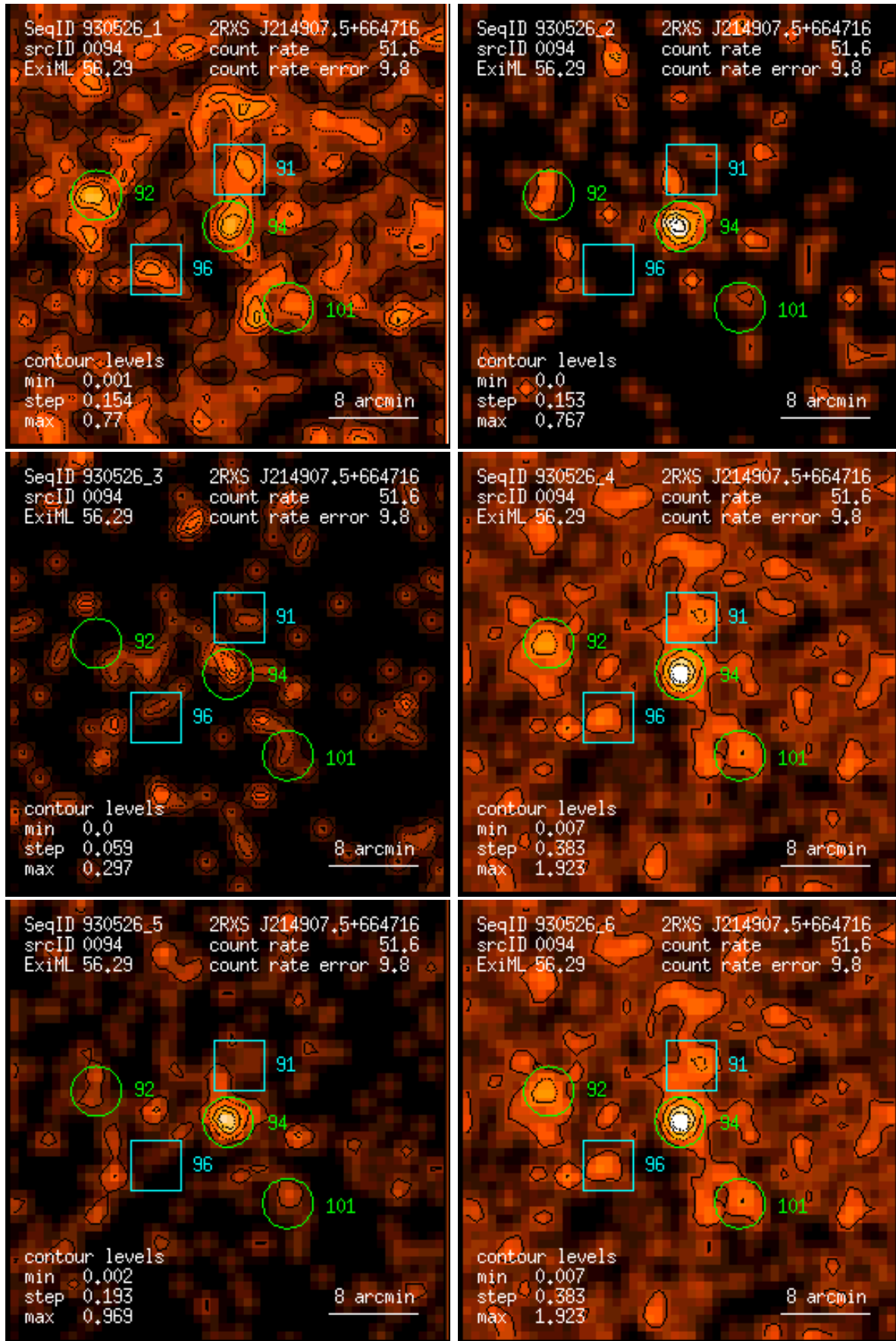
Figure 94: RASS 930526: detection 0094: band rate images, Gaussian filter: (1) PSPC channels 11 – 41, (2) 52 – 90, (3) 91 – 201, (4) 11 – 235, (5) 52 – 201, (6) 11 – 201. Broad band rates in counts/ks. Band rate contour levels in counts/ks/arcmin 2 .
