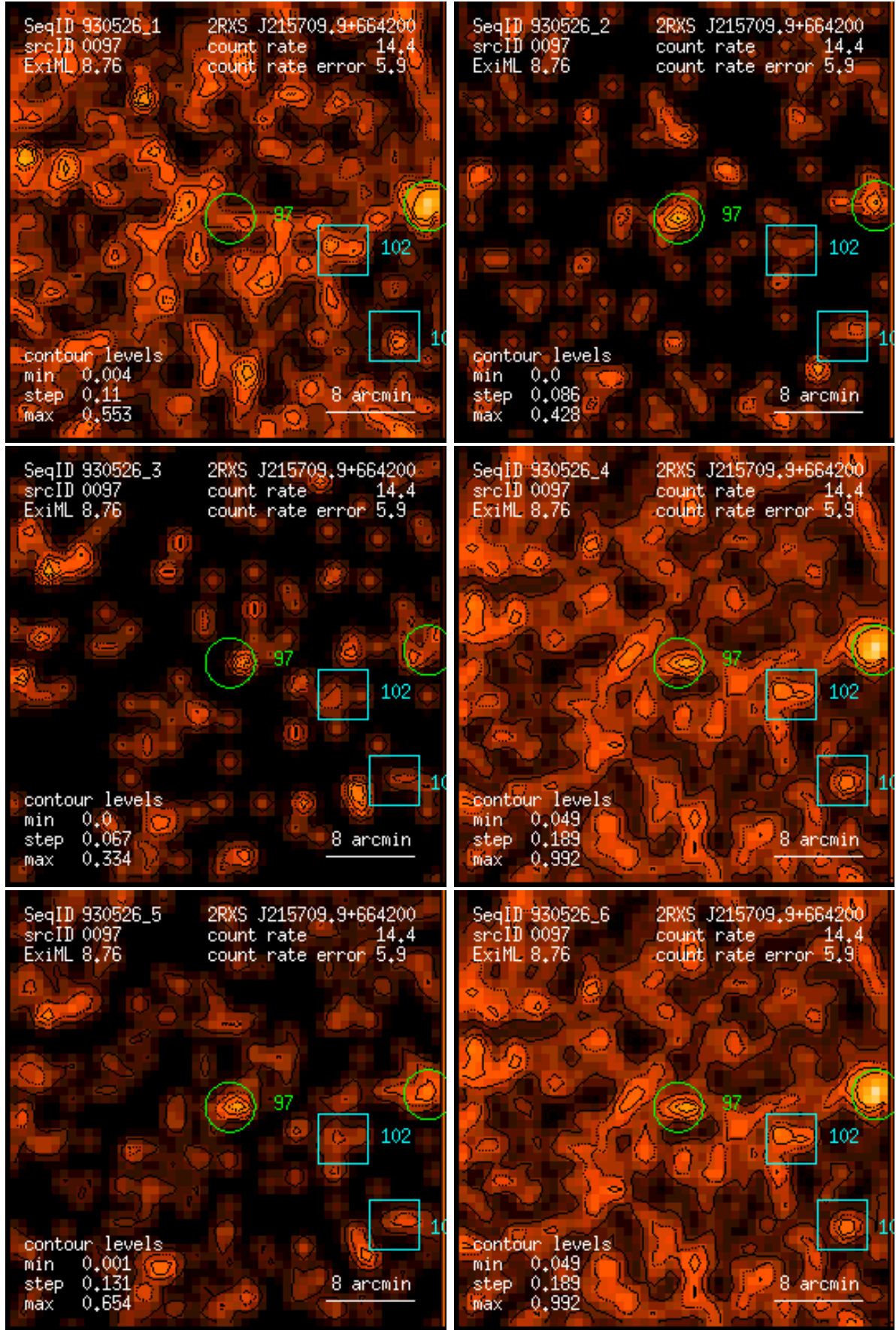
Figure 97: RASS 930526: detection 0097: band rate images, Gaussian filter: (1) PSPC channels 11 – 41, (2) 52 – 90, (3) 91 – 201, (4) 11 – 235, (5) 52 – 201, (6) 11 – 201. Broad band rates in counts/ks. Band rate contour levels in counts/ks/arcmin 2 .
