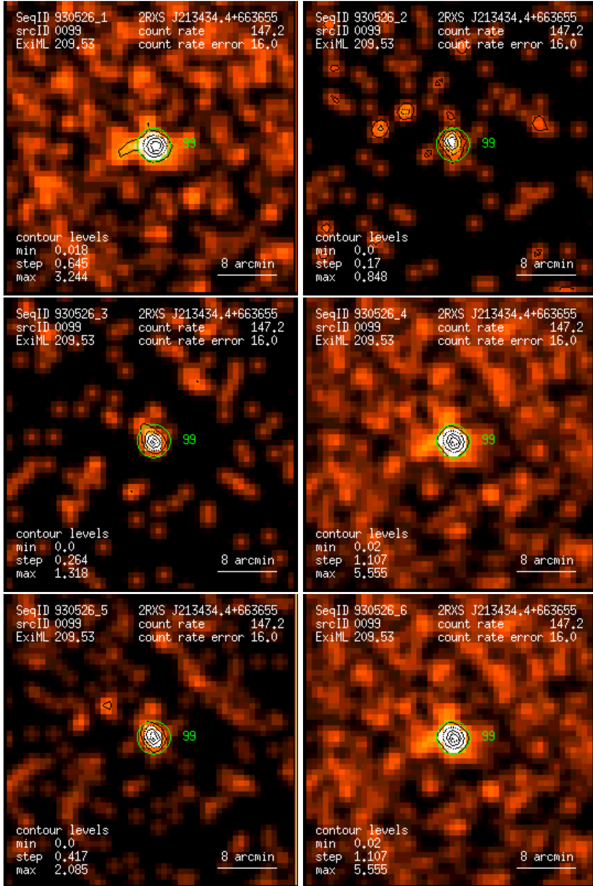
Figure 99: RASS 930526: detection 0099: band rate images, Gaussian filter: (1) PSPC channels 11 – 41, (2) 52 – 90, (3) 91 – 201, (4) 11 – 235, (5) 52 – 201, (6) 11 – 201. Broad band rates in counts/ks. Band rate contour levels in counts/ks/arcmin 2 .
