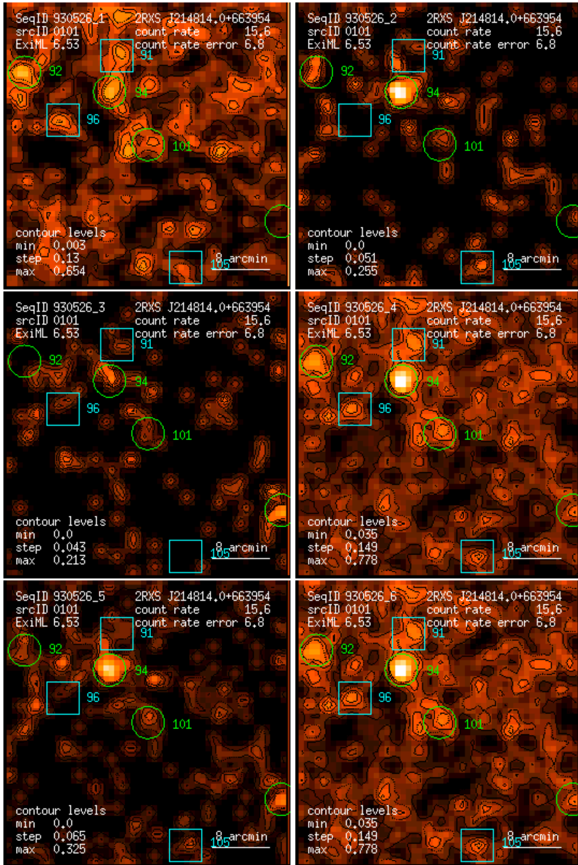
Figure 101: RASS 930526: detection 0101: band rate images, Gaussian filter: (1) PSPC channels 11 – 41, (2) 52 – 90, (3) 91 – 201, (4) 11 – 235, (5) 52 – 201, (6) 11 – 201. Broad band rates in counts/ks. Band rate contour levels in counts/ks/arcmin 2 .
