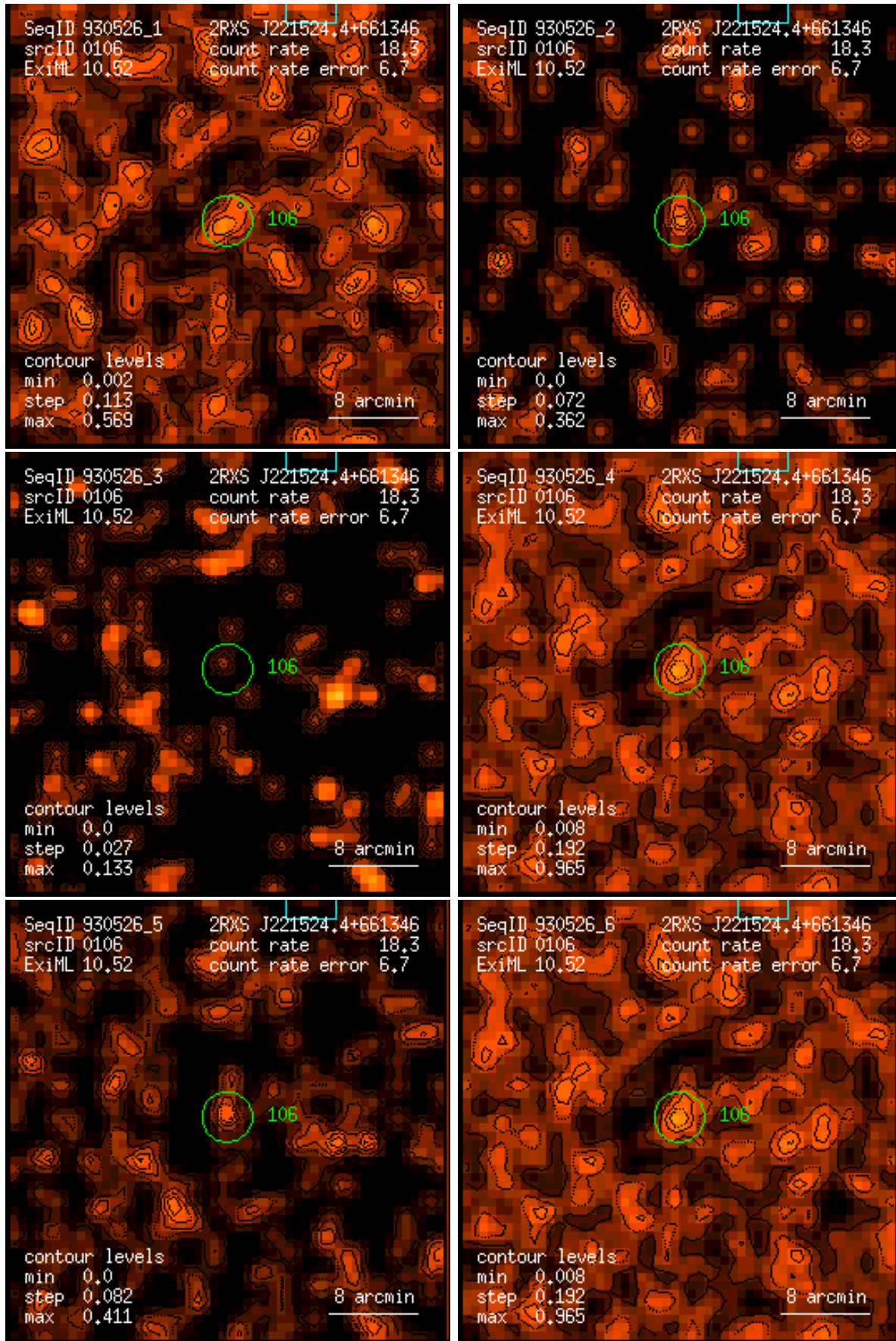
Figure 106: RASS 930526: detection 0106: band rate images, Gaussian filter: (1) PSPC channels 11 – 41, (2) 52 – 90, (3) 91 – 201, (4) 11 – 235, (5) 52 – 201, (6) 11 – 201. Broad band rates in counts/ks. Band rate contour levels in counts/ks/arcmin 2 .
