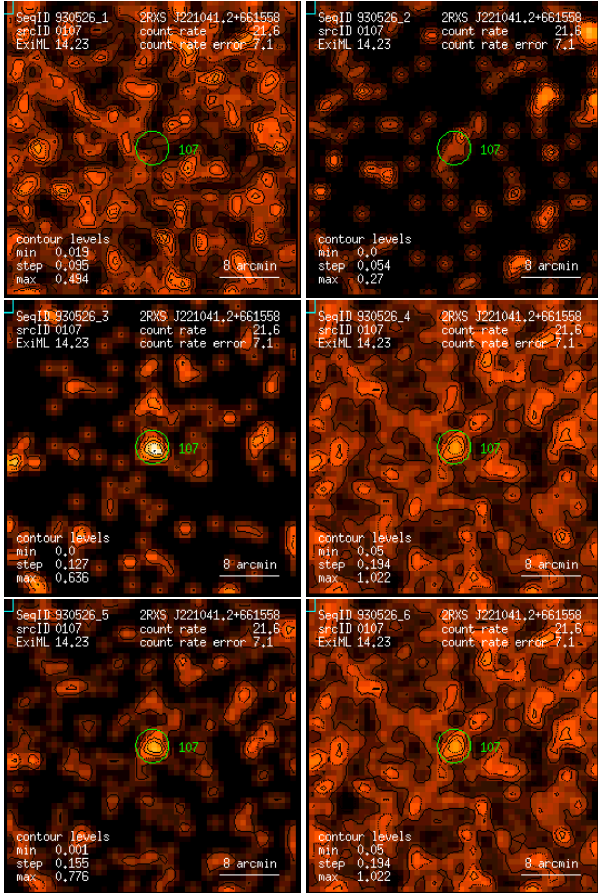
Figure 107: RASS 930526: detection 0107: band rate images, Gaussian filter: (1) PSPC channels 11 – 41, (2) 52 – 90, (3) 91 – 201, (4) 11 – 235, (5) 52 – 201, (6) 11 – 201. Broad band rates in counts/ks. Band rate contour levels in counts/ks/arcmin 2 .
