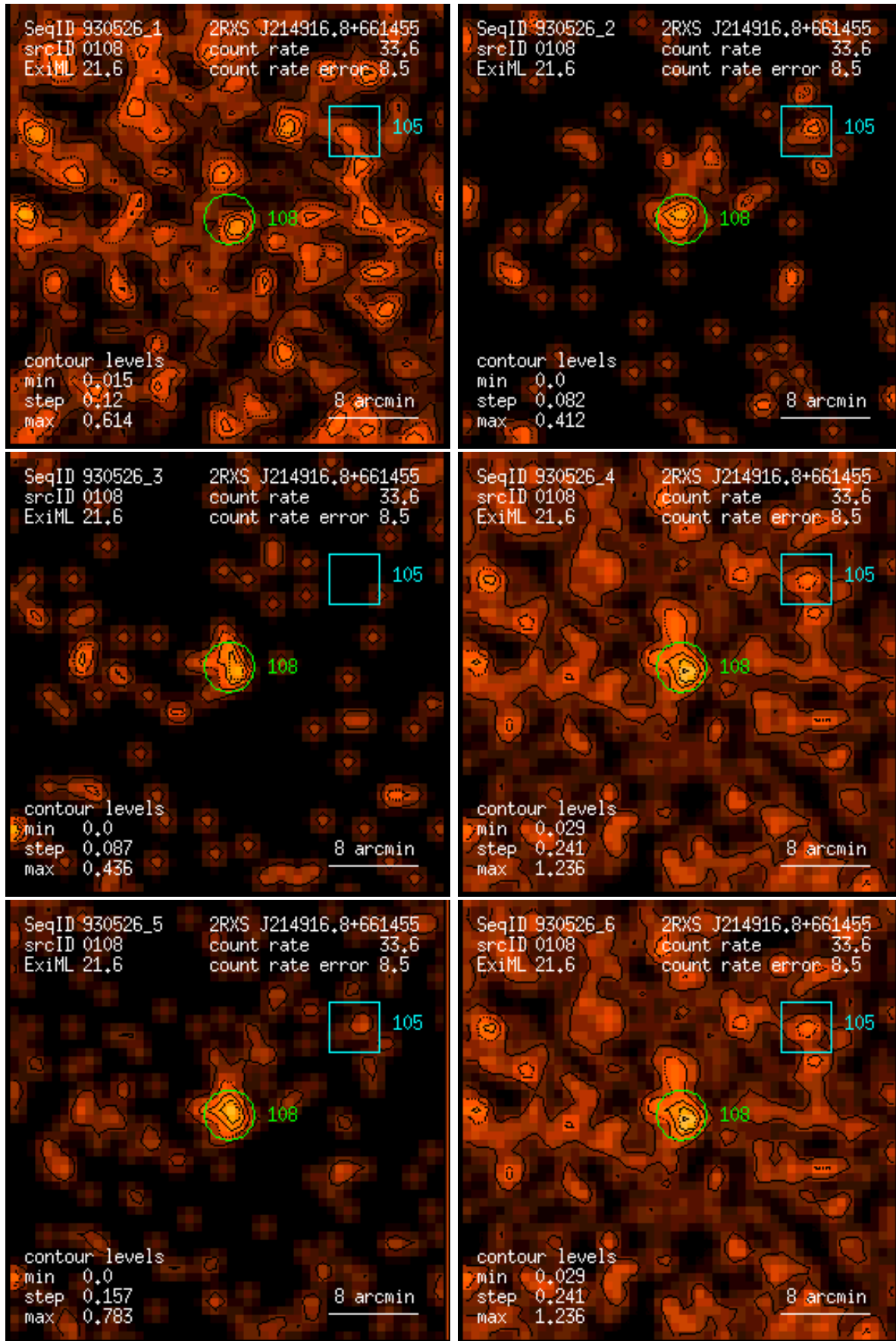
Figure 108: RASS 930526: detection 0108: band rate images, Gaussian filter: (1) PSPC channels 11 – 41, (2) 52 – 90, (3) 91 – 201, (4) 11 – 235, (5) 52 – 201, (6) 11 – 201. Broad band rates in counts/ks. Band rate contour levels in counts/ks/arcmin 2 .
