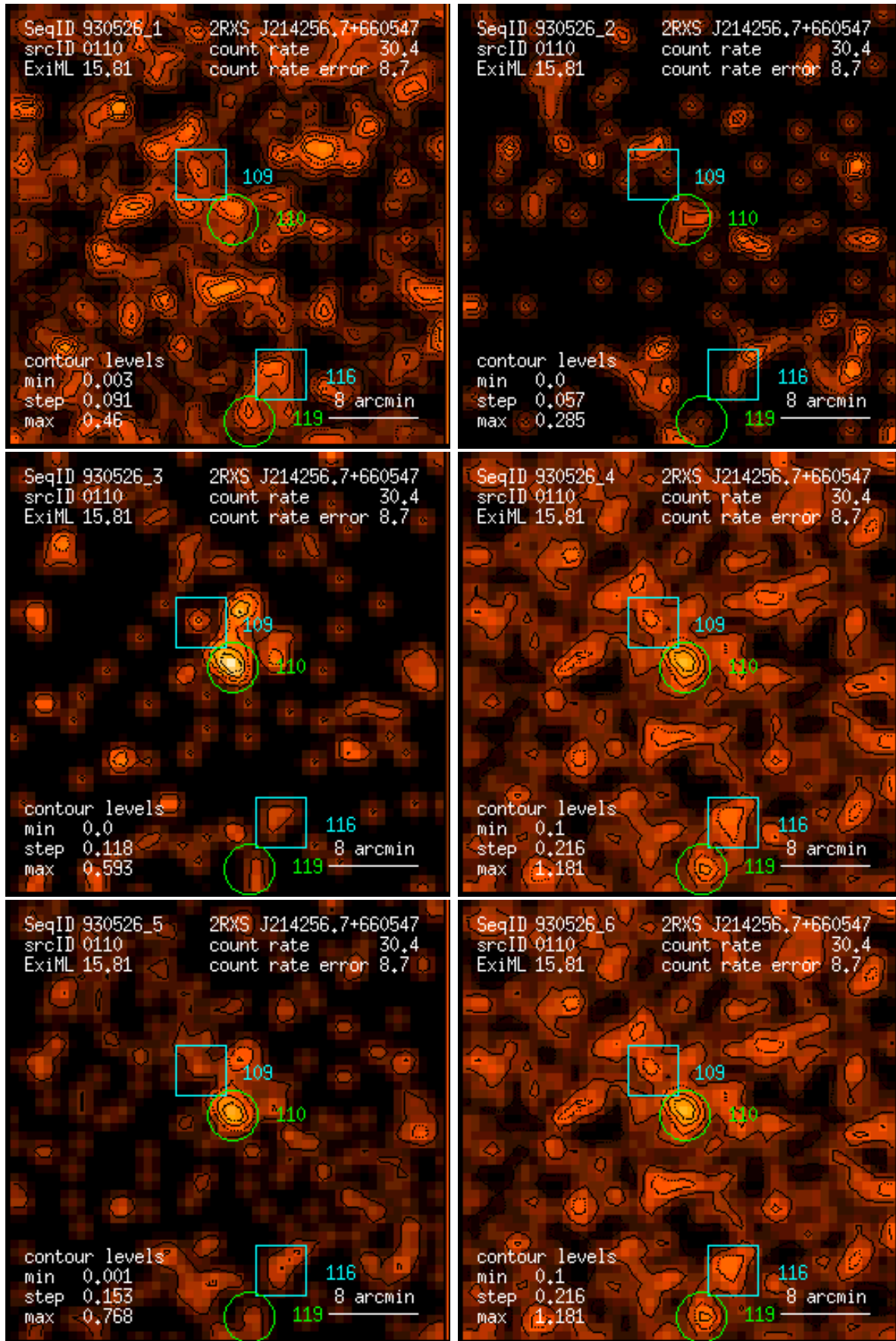
Figure 110: RASS 930526: detection 0110: band rate images, Gaussian filter: (1) PSPC channels 11 – 41, (2) 52 – 90, (3) 91 – 201, (4) 11 – 235, (5) 52 – 201, (6) 11 – 201. Broad band rates in counts/ks. Band rate contour levels in counts/ks/arcmin 2 .
