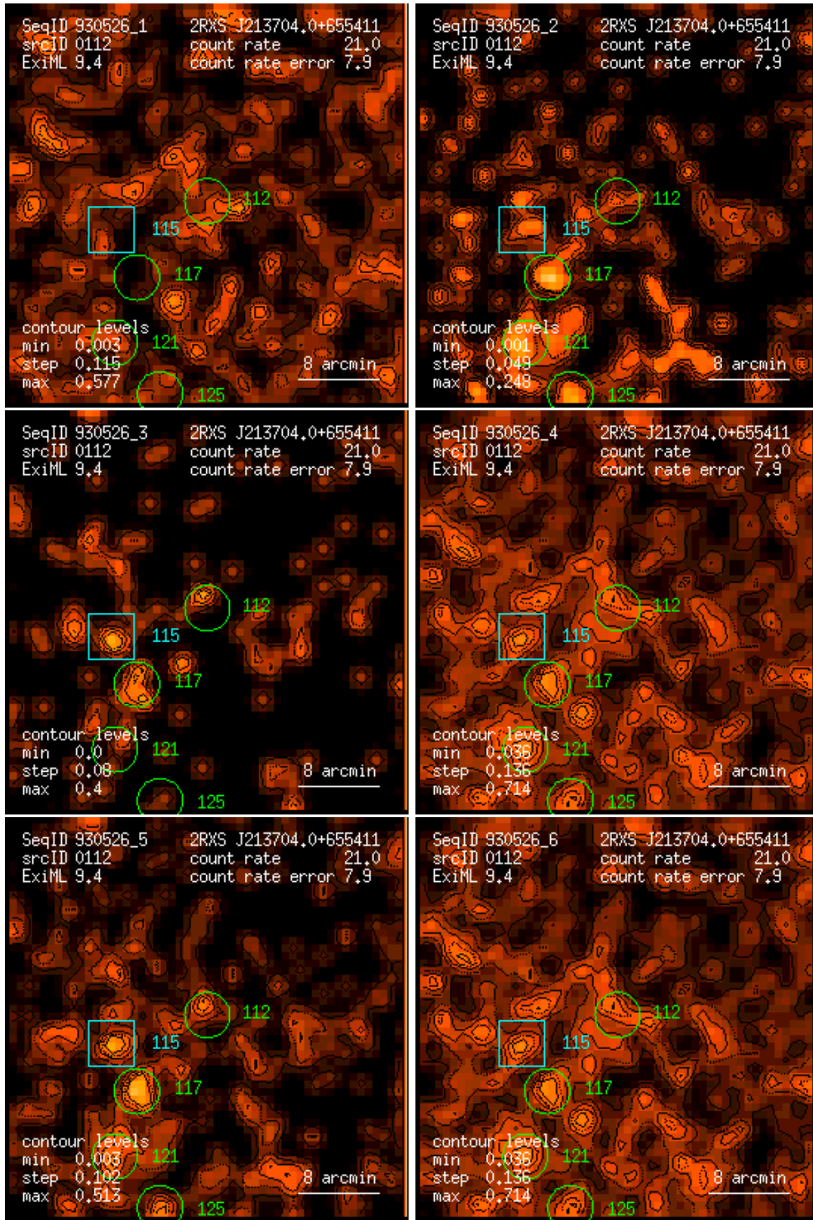
Figure 112: RASS 930526: detection 0112: band rate images, Gaussian filter: (1) PSPC channels 11 – 41, (2) 52 – 90, (3) 91 – 201, (4) 11 – 235, (5) 52 – 201, (6) 11 – 201. Broad band rates in counts/ks. Band rate contour levels in counts/ks/arcmin 2 .
