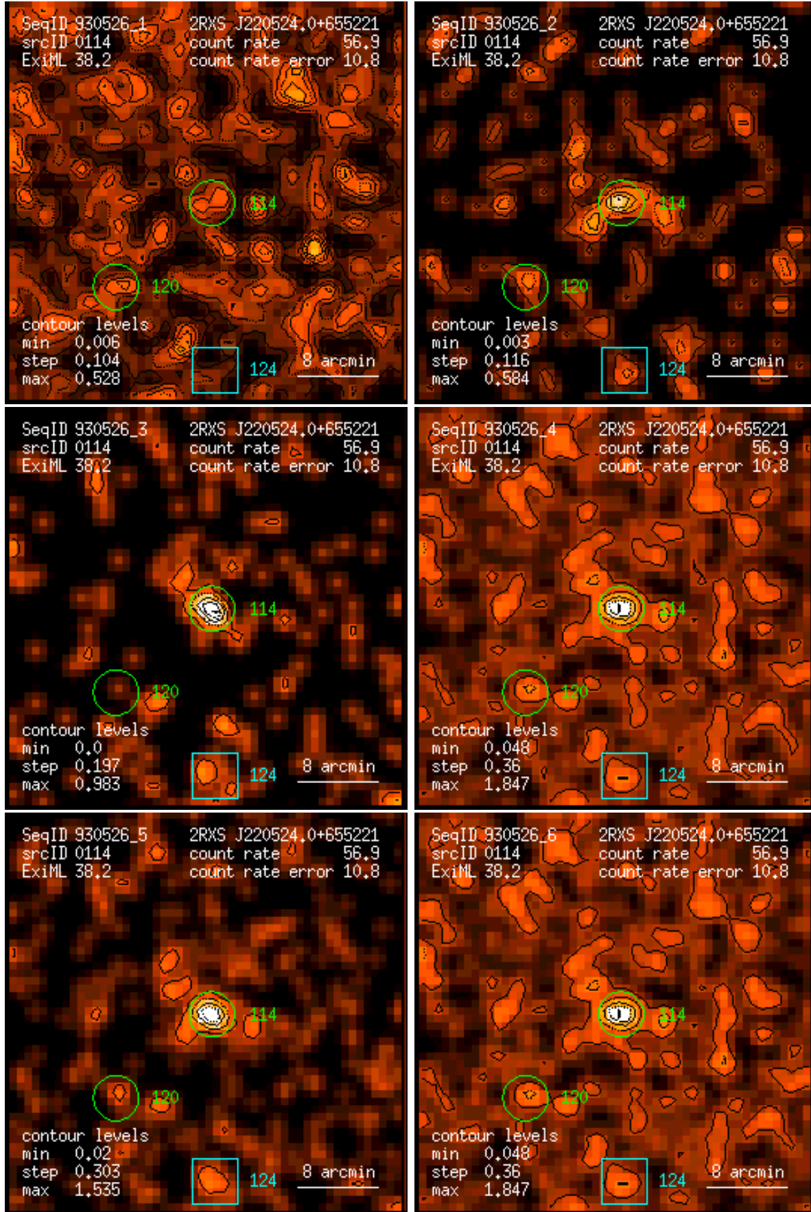
Figure 114: RASS 930526: detection 0114: band rate images, Gaussian filter: (1) PSPC channels 11 – 41, (2) 52 – 90, (3) 91 – 201, (4) 11 – 235, (5) 52 – 201, (6) 11 – 201. Broad band rates in counts/ks. Band rate contour levels in counts/ks/arcmin 2 .
