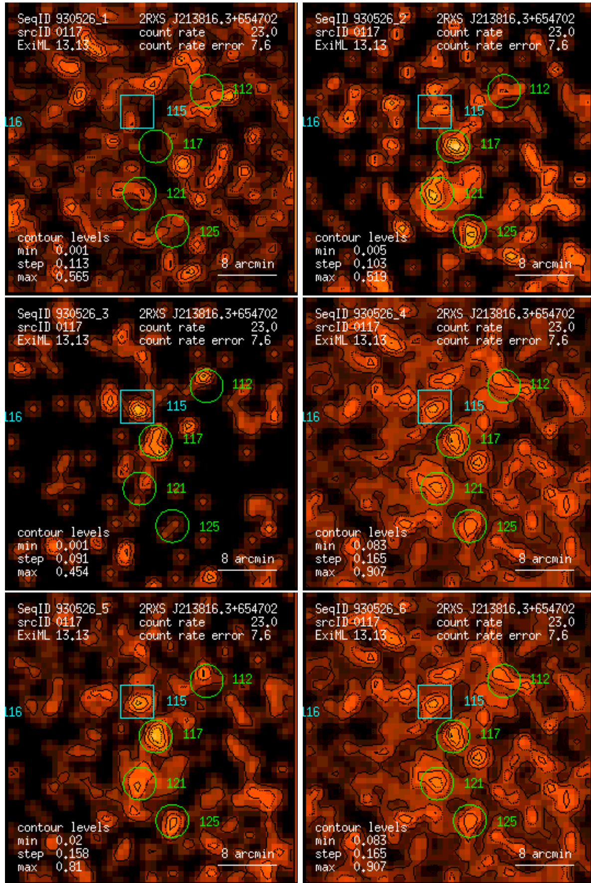
Figure 117: RASS 930526: detection 0117: band rate images, Gaussian filter: (1) PSPC channels 11 – 41, (2) 52 – 90, (3) 91 – 201, (4) 11 – 235, (5) 52 – 201, (6) 11 – 201. Broad band rates in counts/ks. Band rate contour levels in counts/ks/arcmin 2 .
