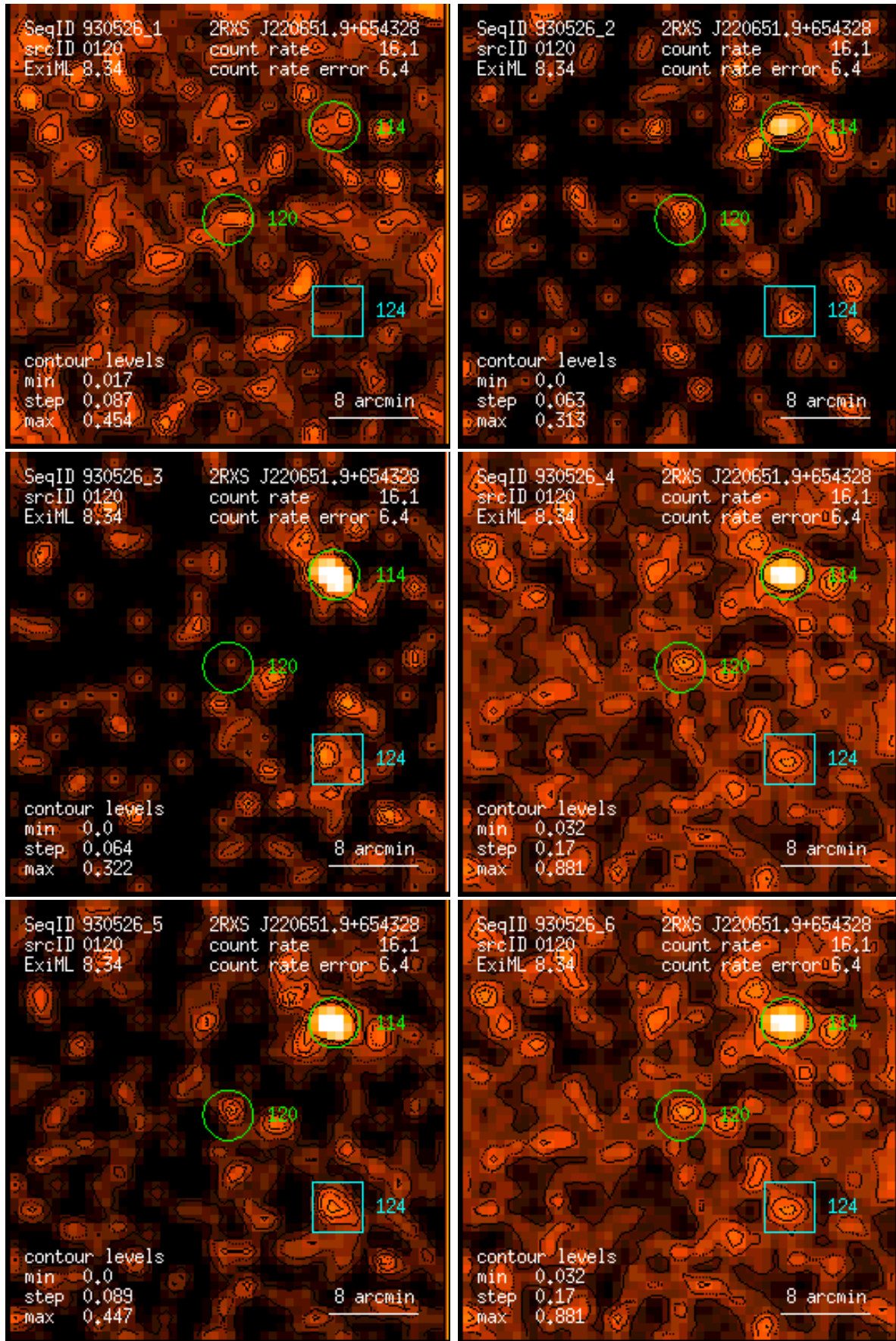
Figure 120: RASS 930526: detection 0120: band rate images, Gaussian filter: (1) PSPC channels 11 – 41, (2) 52 – 90, (3) 91 – 201, (4) 11 – 235, (5) 52 – 201, (6) 11 – 201. Broad band rates in counts/ks. Band rate contour levels in counts/ks/arcmin 2 .
