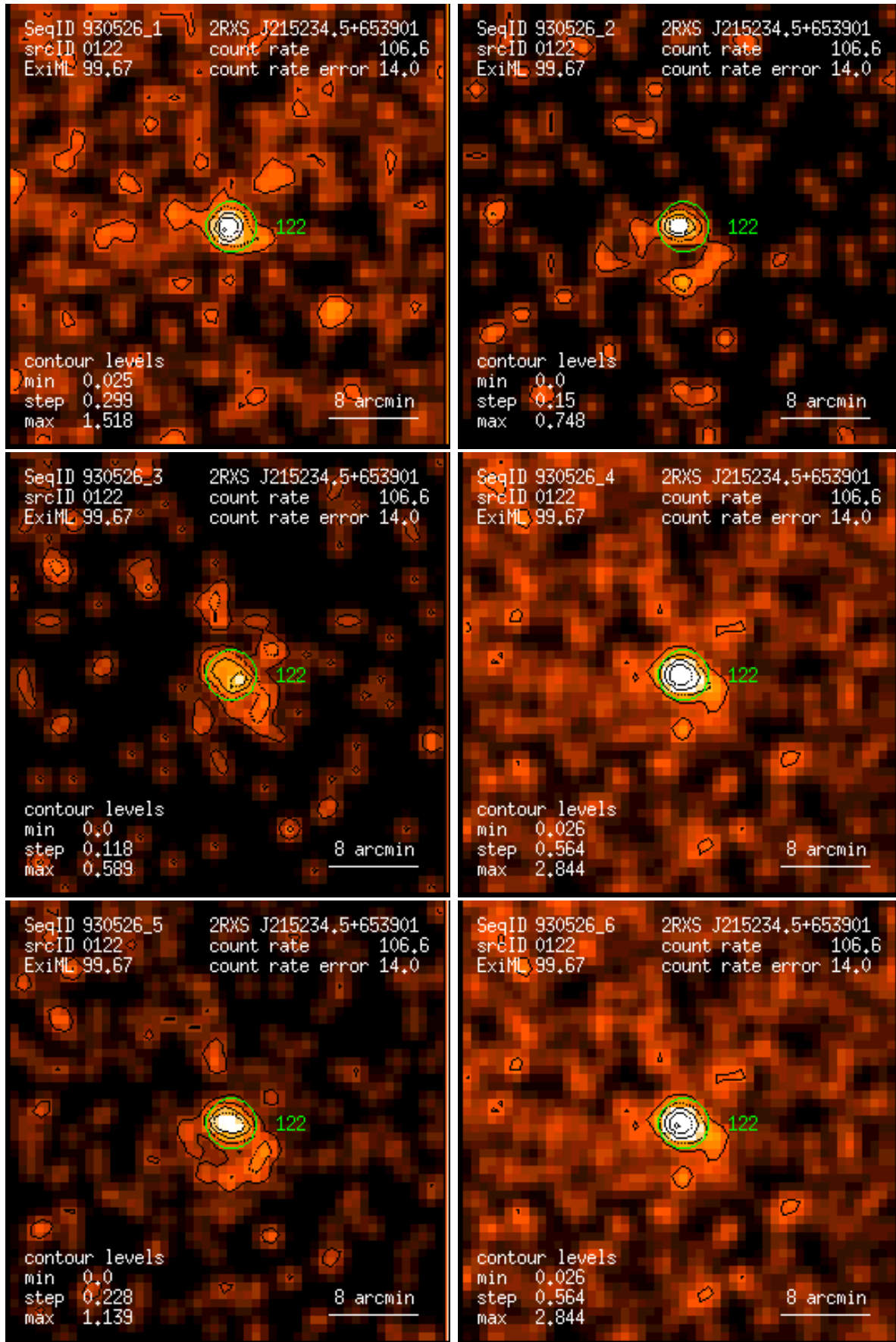
Figure 122: RASS 930526: detection 0122: band rate images, Gaussian filter: (1) PSPC channels 11 – 41, (2) 52 – 90, (3) 91 – 201, (4) 11 – 235, (5) 52 – 201, (6) 11 – 201. Broad band rates in counts/ks. Band rate contour levels in counts/ks/arcmin 2 .
