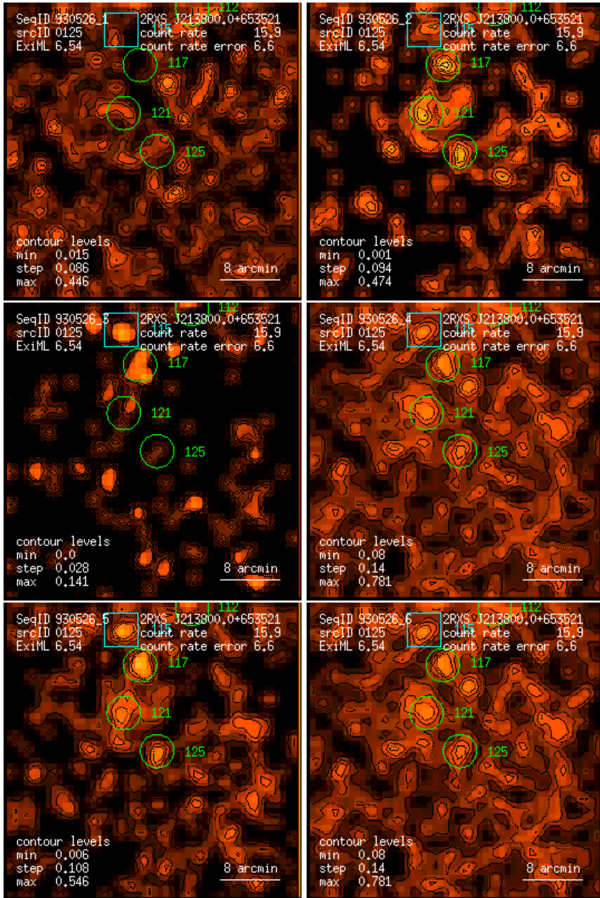
Figure 125: RASS 930526: detection 0125: band rate images, Gaussian filter: (1) PSPC channels 11 – 41, (2) 52 – 90, (3) 91 – 201, (4) 11 – 235, (5) 52 – 201, (6) 11 – 201. Broad band rates in counts/ks. Band rate contour levels in counts/ks/arcmin 2 .
