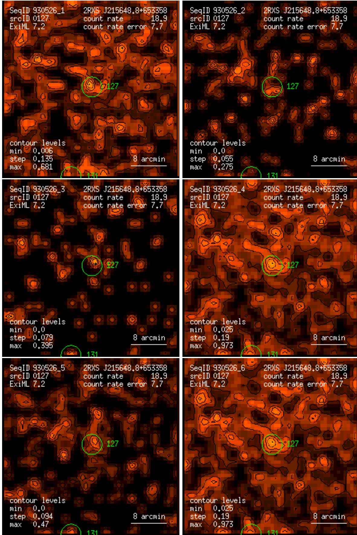
Figure 127: RASS 930526: detection 0127: band rate images, Gaussian filter: (1) PSPC channels 11 – 41, (2) 52 – 90, (3) 91 – 201, (4) 11 – 235, (5) 52 – 201, (6) 11 – 201. Broad band rates in counts/ks. Band rate contour levels in counts/ks/arcmin 2 .
