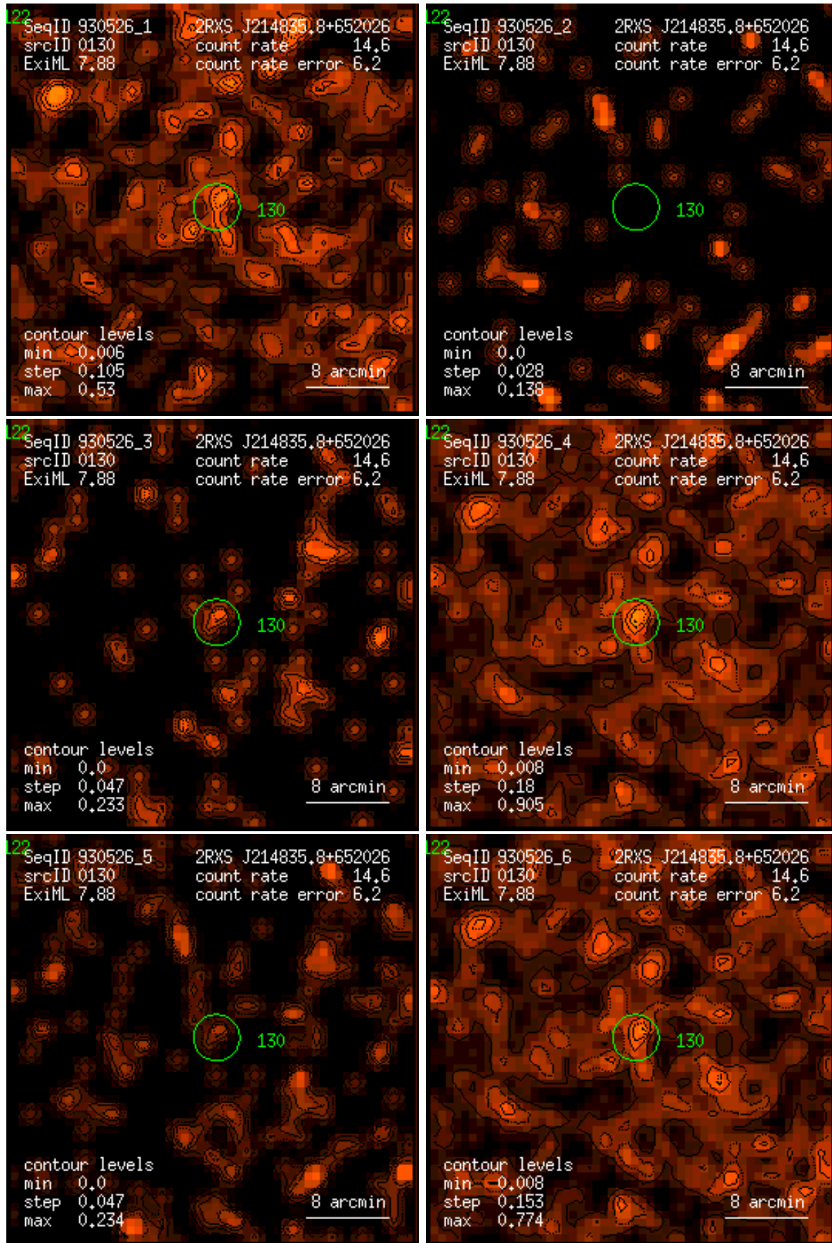
Figure 130: RASS 930526: detection 0130: band rate images, Gaussian filter: (1) PSPC channels 11 – 41, (2) 52 – 90, (3) 91 – 201, (4) 11 – 235, (5) 52 – 201, (6) 11 – 201. Broad band rates in counts/ks. Band rate contour levels in counts/ks/arcmin 2 .
