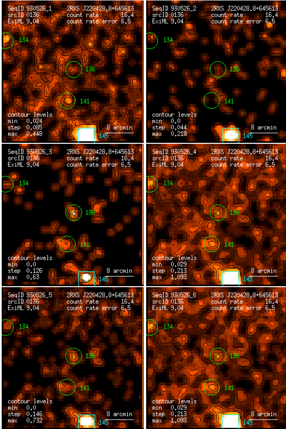
Figure 136: RASS 930526: detection 0136: band rate images, Gaussian filter: (1) PSPC channels 11 – 41, (2) 52 – 90, (3) 91 – 201, (4) 11 – 235, (5) 52 – 201, (6) 11 – 201. Broad band rates in counts/ks. Band rate contour levels in counts/ks/arcmin 2 .
