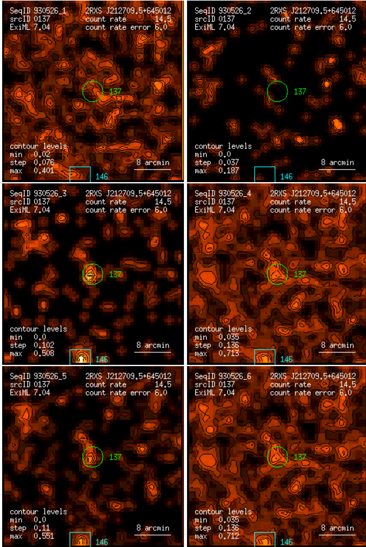
Figure 137: RASS 930526: detection 0137: band rate images, Gaussian filter: (1) PSPC channels 11 – 41, (2) 52 – 90, (3) 91 – 201, (4) 11 – 235, (5) 52 – 201, (6) 11 – 201. Broad band rates in counts/ks. Band rate contour levels in counts/ks/arcmin 2 .
