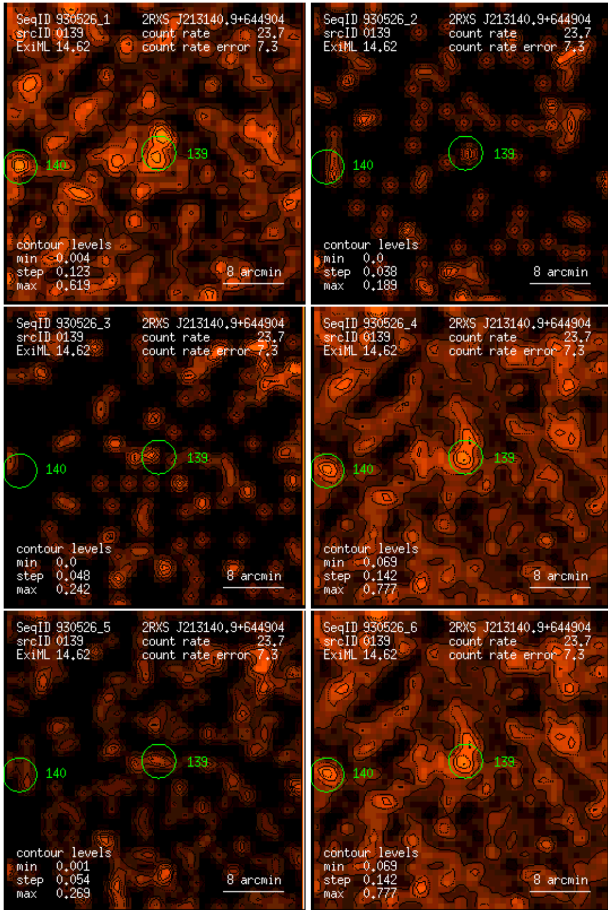
Figure 139: RASS 930526: detection 0139: band rate images, Gaussian filter: (1) PSPC channels 11 – 41, (2) 52 – 90, (3) 91 – 201, (4) 11 – 235, (5) 52 – 201, (6) 11 – 201. Broad band rates in counts/ks. Band rate contour levels in counts/ks/arcmin 2 .
