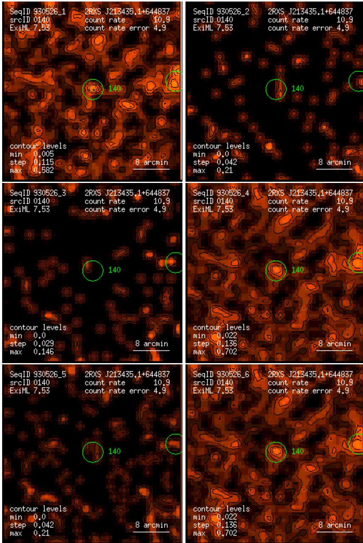
Figure 140: RASS 930526: detection 0140: band rate images, Gaussian filter: (1) PSPC channels 11 – 41, (2) 52 – 90, (3) 91 – 201, (4) 11 – 235, (5) 52 – 201, (6) 11 – 201. Broad band rates in counts/ks. Band rate contour levels in counts/ks/arcmin 2 .
