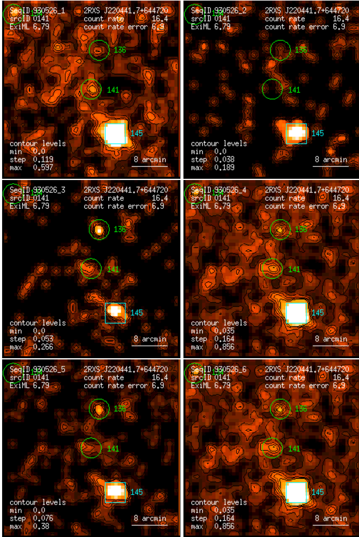
Figure 141: RASS 930526: detection 0141: band rate images, Gaussian filter: (1) PSPC channels 11 – 41, (2) 52 – 90, (3) 91 – 201, (4) 11 – 235, (5) 52 – 201, (6) 11 – 201. Broad band rates in counts/ks. Band rate contour levels in counts/ks/arcmin 2 .
