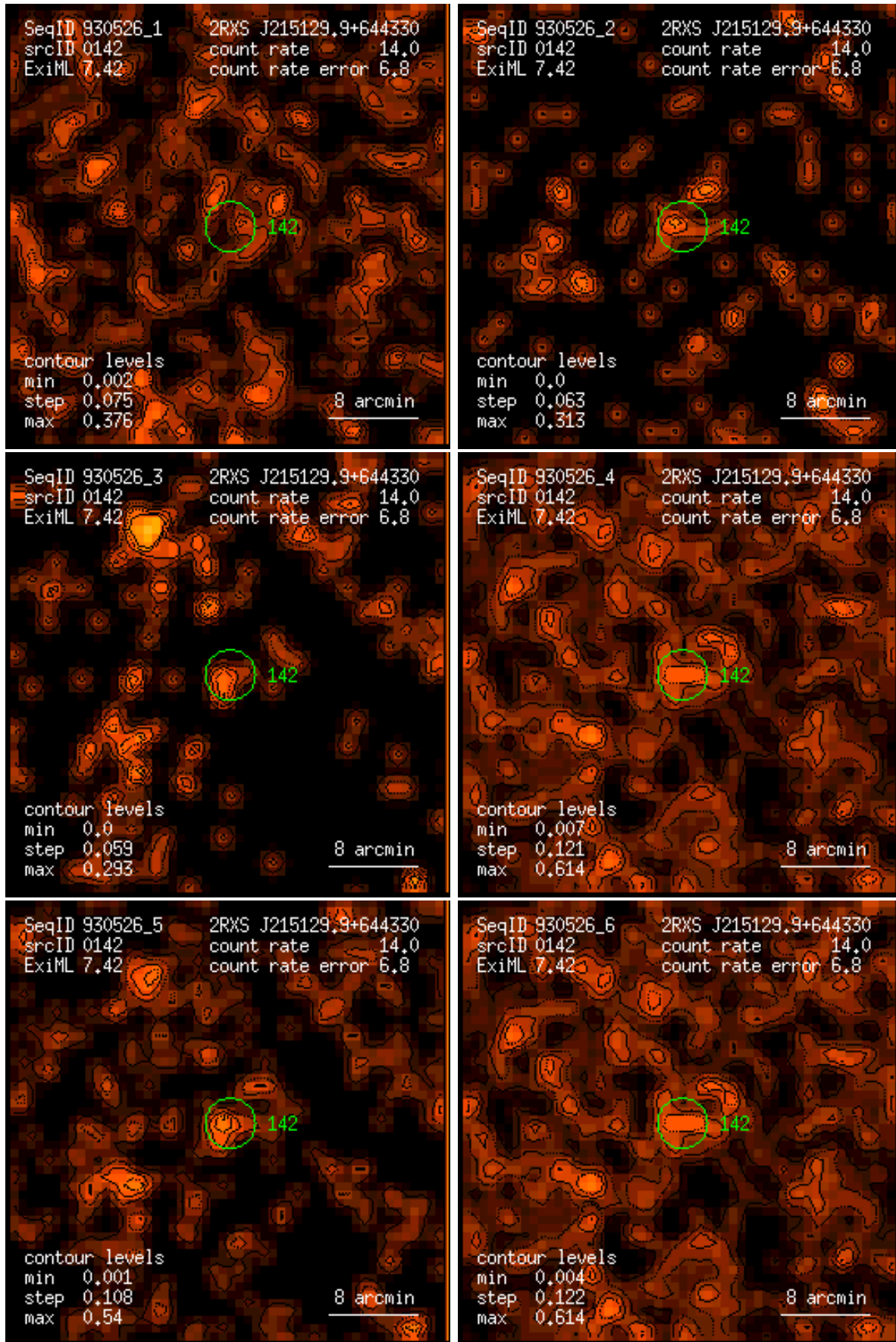
Figure 142: RASS 930526: detection 0142: band rate images, Gaussian filter: (1) PSPC channels 11 – 41, (2) 52 – 90, (3) 91 – 201, (4) 11 – 235, (5) 52 – 201, (6) 11 – 201. Broad band rates in counts/ks. Band rate contour levels in counts/ks/arcmin 2 .
