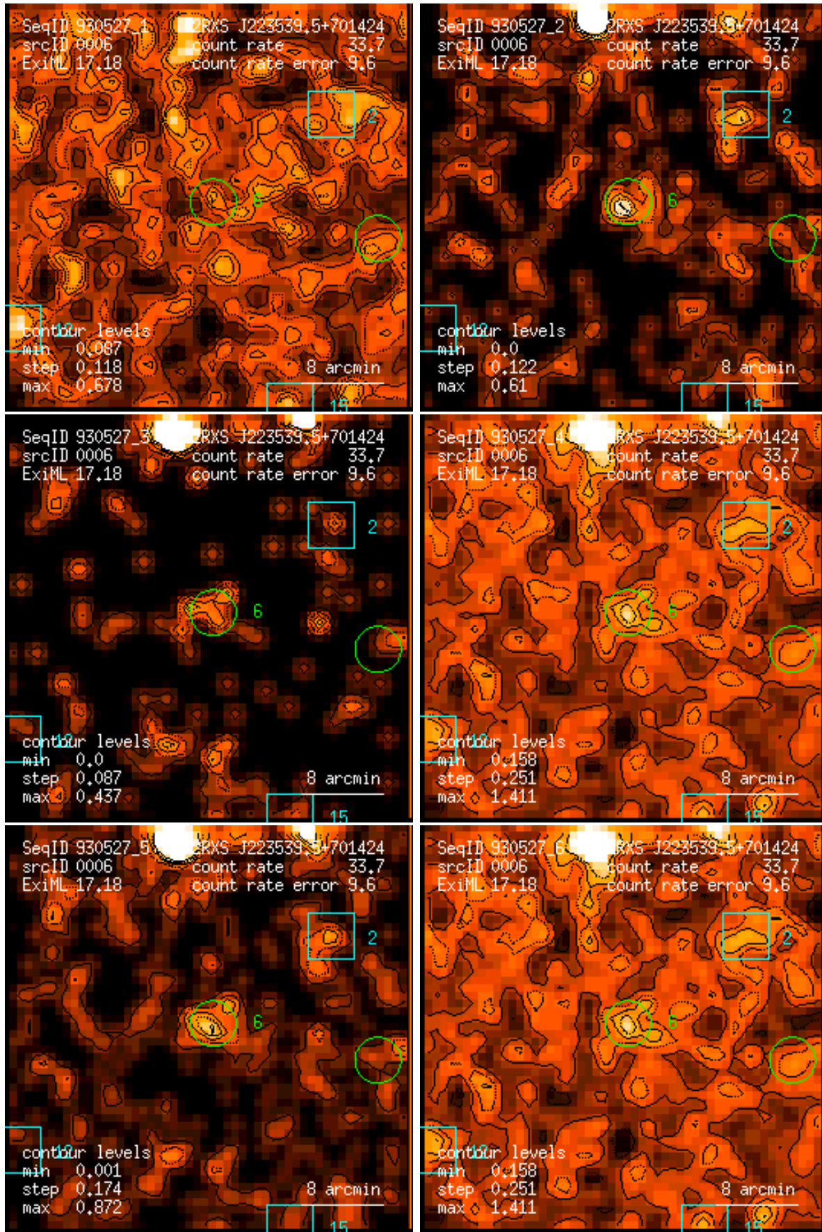
Figure 6: RASS 930527: detection 0006: band rate images, Gaussian filter: (1) PSPC channels 11 – 41, (2) 52 – 90, (3) 91 – 201, (4) 11 – 235, (5) 52 – 201, (6) 11 – 201. Broad band rates in counts/ks. Band rate contour levels in counts/ks/arcmin 2 .
