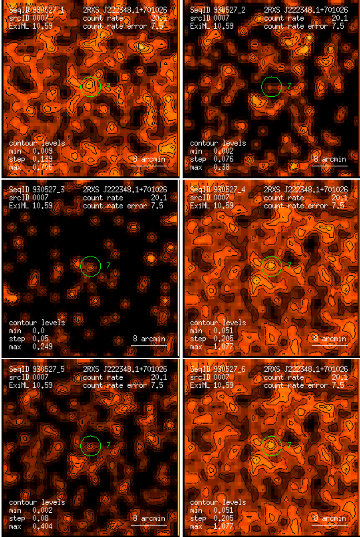
Figure 7: RASS 930527: detection 0007: band rate images, Gaussian filter: (1) PSPC channels 11 – 41, (2) 52 – 90, (3) 91 – 201, (4) 11 – 235, (5) 52 – 201, (6) 11 – 201. Broad band rates in counts/ks. Band rate contour levels in counts/ks/arcmin 2 .
