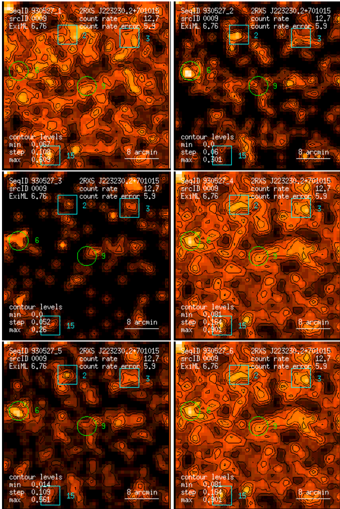
Figure 9: RASS 930527: detection 0009: band rate images, Gaussian filter: (1) PSPC channels 11 – 41, (2) 52 – 90, (3) 91 – 201, (4) 11 – 235, (5) 52 – 201, (6) 11 – 201. Broad band rates in counts/ks. Band rate contour levels in counts/ks/arcmin 2 .
