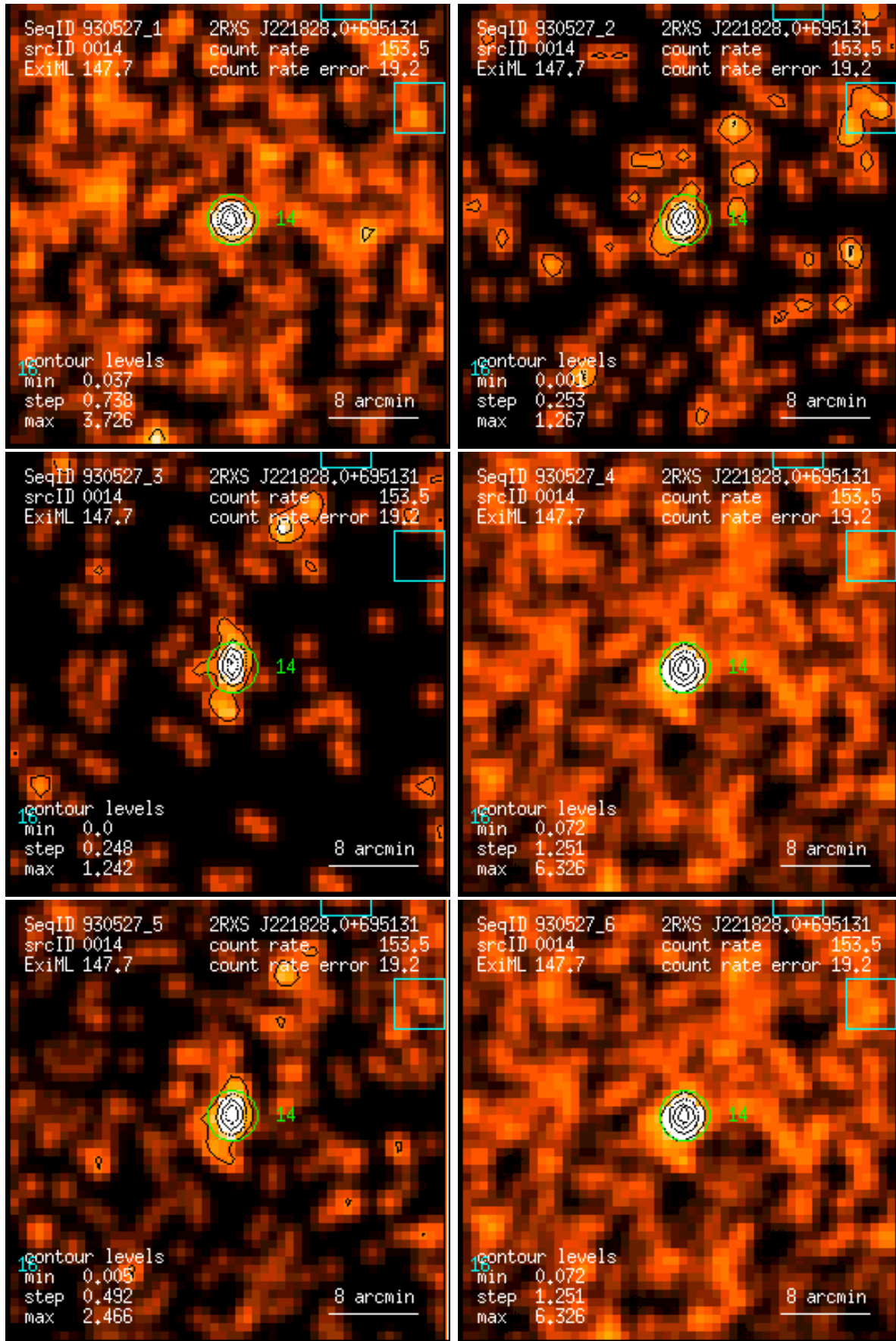
Figure 14: RASS 930527: detection 0014: band rate images, Gaussian filter: (1) PSPC channels 11 – 41, (2) 52 – 90, (3) 91 – 201, (4) 11 – 235, (5) 52 – 201, (6) 11 – 201. Broad band rates in counts/ks. Band rate contour levels in counts/ks/arcmin 2 .
