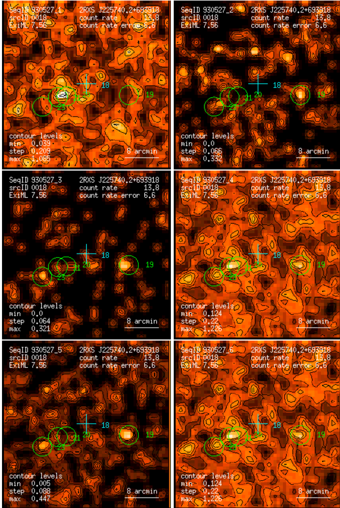
Figure 18: RASS 930527: detection 0018: band rate images, Gaussian filter: (1) PSPC channels 11 – 41, (2) 52 – 90, (3) 91 – 201, (4) 11 – 235, (5) 52 – 201, (6) 11 – 201. Broad band rates in counts/ks. Band rate contour levels in counts/ks/arcmin 2 .
