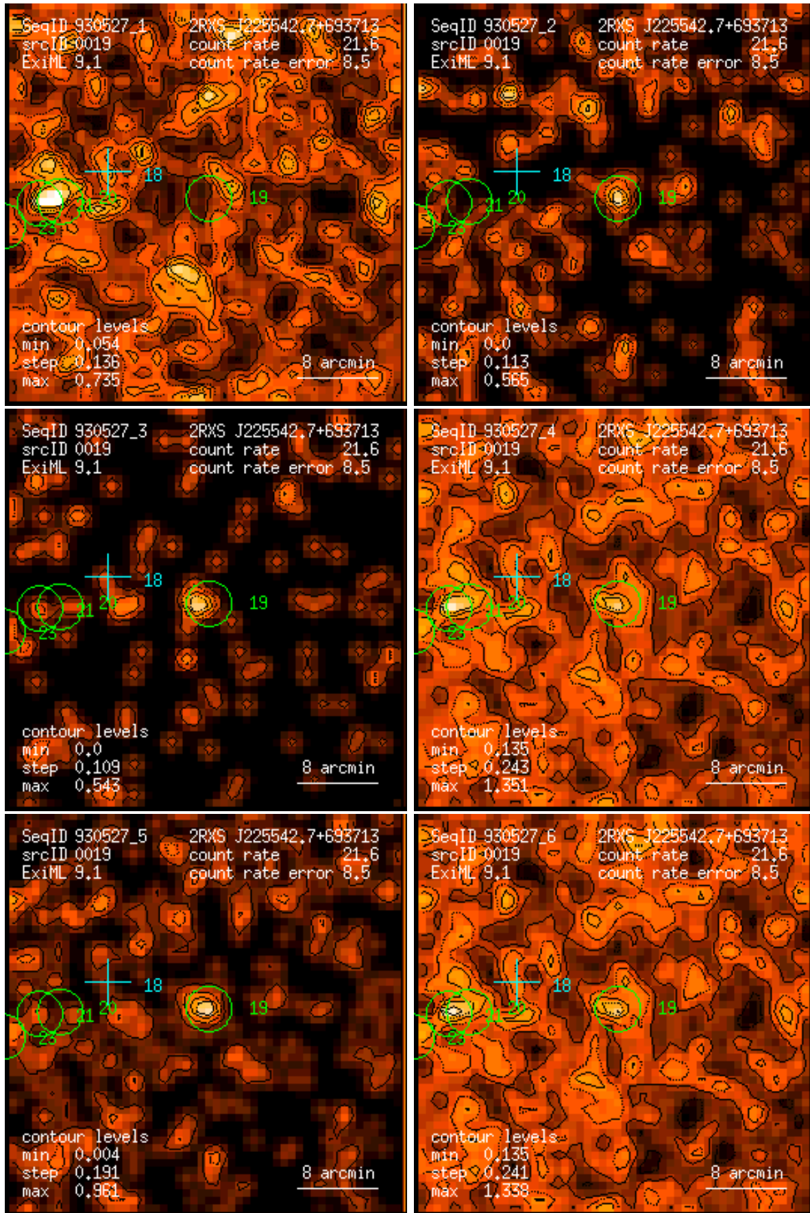
Figure 19: RASS 930527: detection 0019: band rate images, Gaussian filter: (1) PSPC channels 11 – 41, (2) 52 – 90, (3) 91 – 201, (4) 11 – 235, (5) 52 – 201, (6) 11 – 201. Broad band rates in counts/ks. Band rate contour levels in counts/ks/arcmin 2 .
