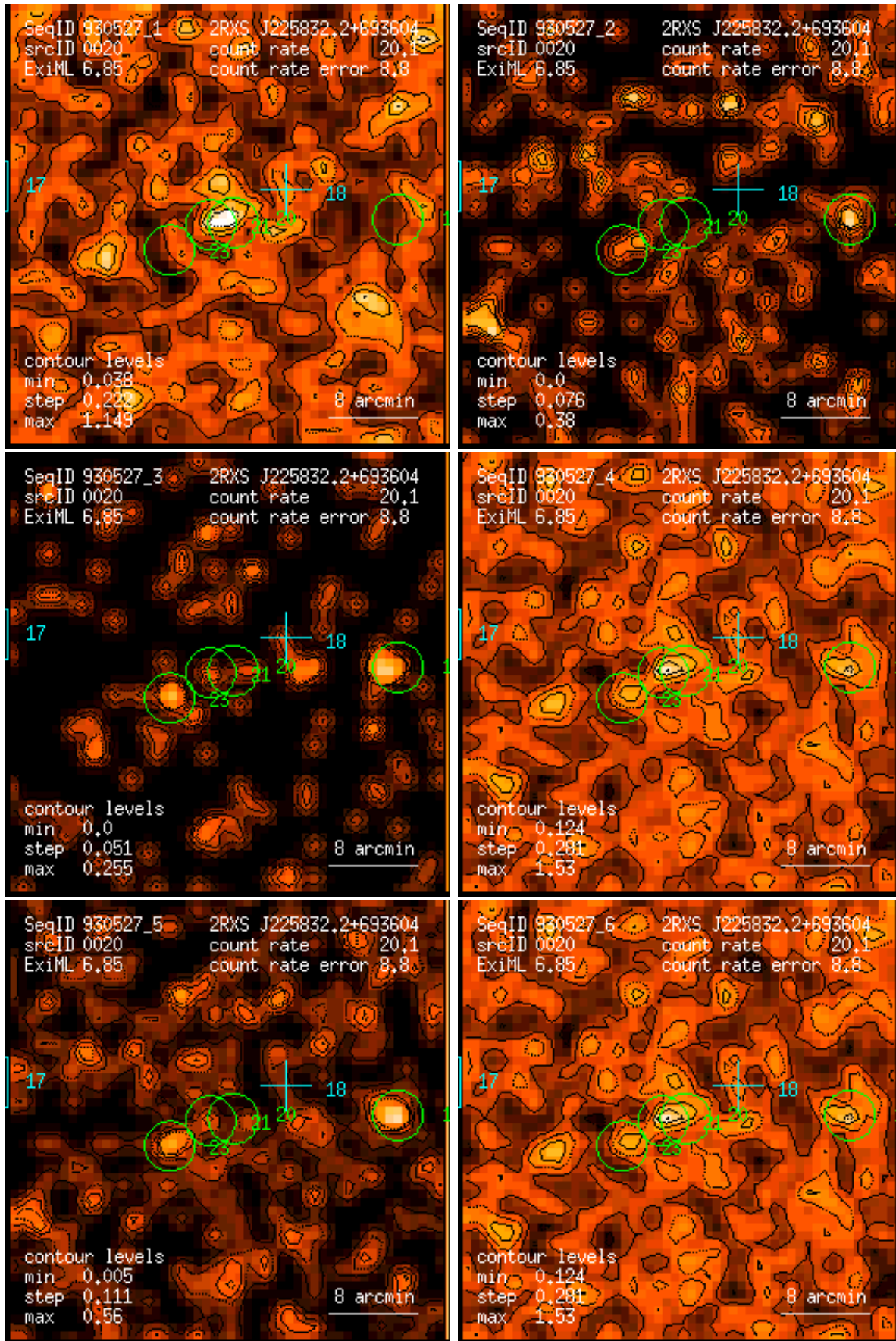
Figure 20: RASS 930527: detection 0020: band rate images, Gaussian filter: (1) PSPC channels 11 – 41, (2) 52 – 90, (3) 91 – 201, (4) 11 – 235, (5) 52 – 201, (6) 11 – 201. Broad band rates in counts/ks. Band rate contour levels in counts/ks/arcmin 2 .
