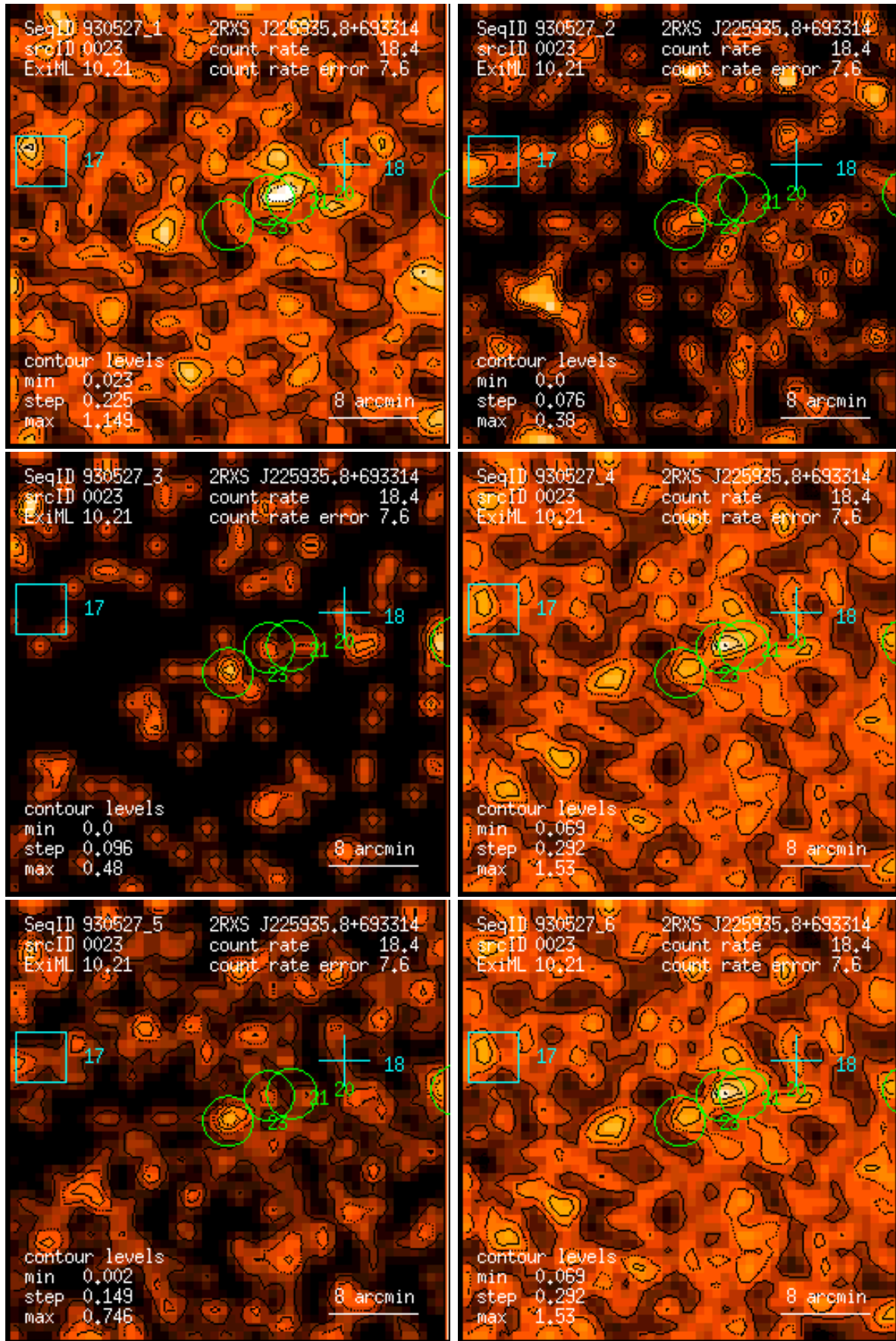
Figure 23: RASS 930527: detection 0023: band rate images, Gaussian filter: (1) PSPC channels 11 – 41, (2) 52 – 90, (3) 91 – 201, (4) 11 – 235, (5) 52 – 201, (6) 11 – 201. Broad band rates in counts/ks. Band rate contour levels in counts/ks/arcmin 2 .
