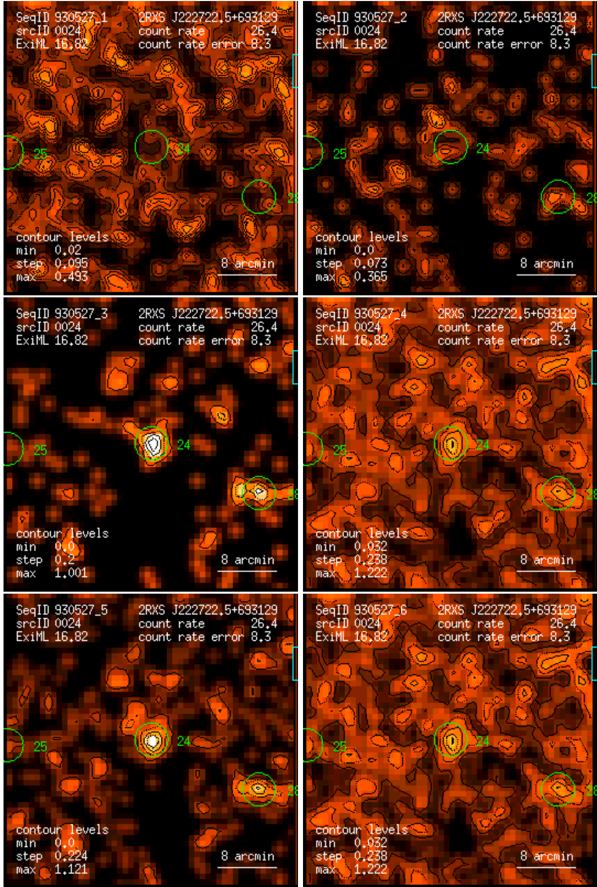
Figure 24: RASS 930527: detection 0024: band rate images, Gaussian filter: (1) PSPC channels 11 – 41, (2) 52 – 90, (3) 91 – 201, (4) 11 – 235, (5) 52 – 201, (6) 11 – 201. Broad band rates in counts/ks. Band rate contour levels in counts/ks/arcmin 2 .
