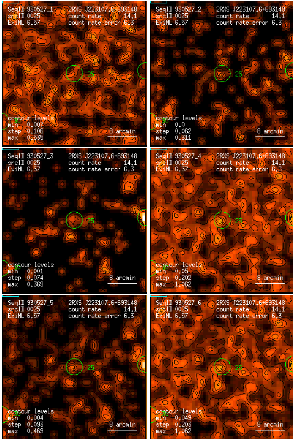
Figure 25: RASS 930527: detection 0025: band rate images, Gaussian filter: (1) PSPC channels 11 – 41, (2) 52 – 90, (3) 91 – 201, (4) 11 – 235, (5) 52 – 201, (6) 11 – 201. Broad band rates in counts/ks. Band rate contour levels in counts/ks/arcmin 2 .
