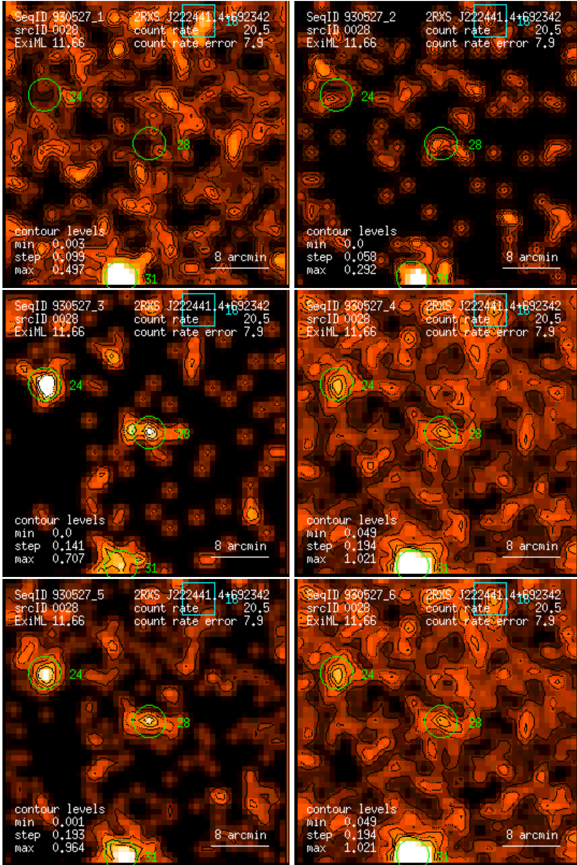
Figure 28: RASS 930527: detection 0028: band rate images, Gaussian filter: (1) PSPC channels 11 – 41, (2) 52 – 90, (3) 91 – 201, (4) 11 – 235, (5) 52 – 201, (6) 11 – 201. Broad band rates in counts/ks. Band rate contour levels in counts/ks/arcmin 2 .
