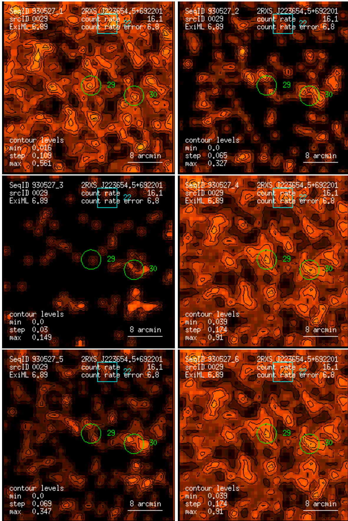
Figure 29: RASS 930527: detection 0029: band rate images, Gaussian filter: (1) PSPC channels 11 – 41, (2) 52 – 90, (3) 91 – 201, (4) 11 – 235, (5) 52 – 201, (6) 11 – 201. Broad band rates in counts/ks. Band rate contour levels in counts/ks/arcmin 2 .
