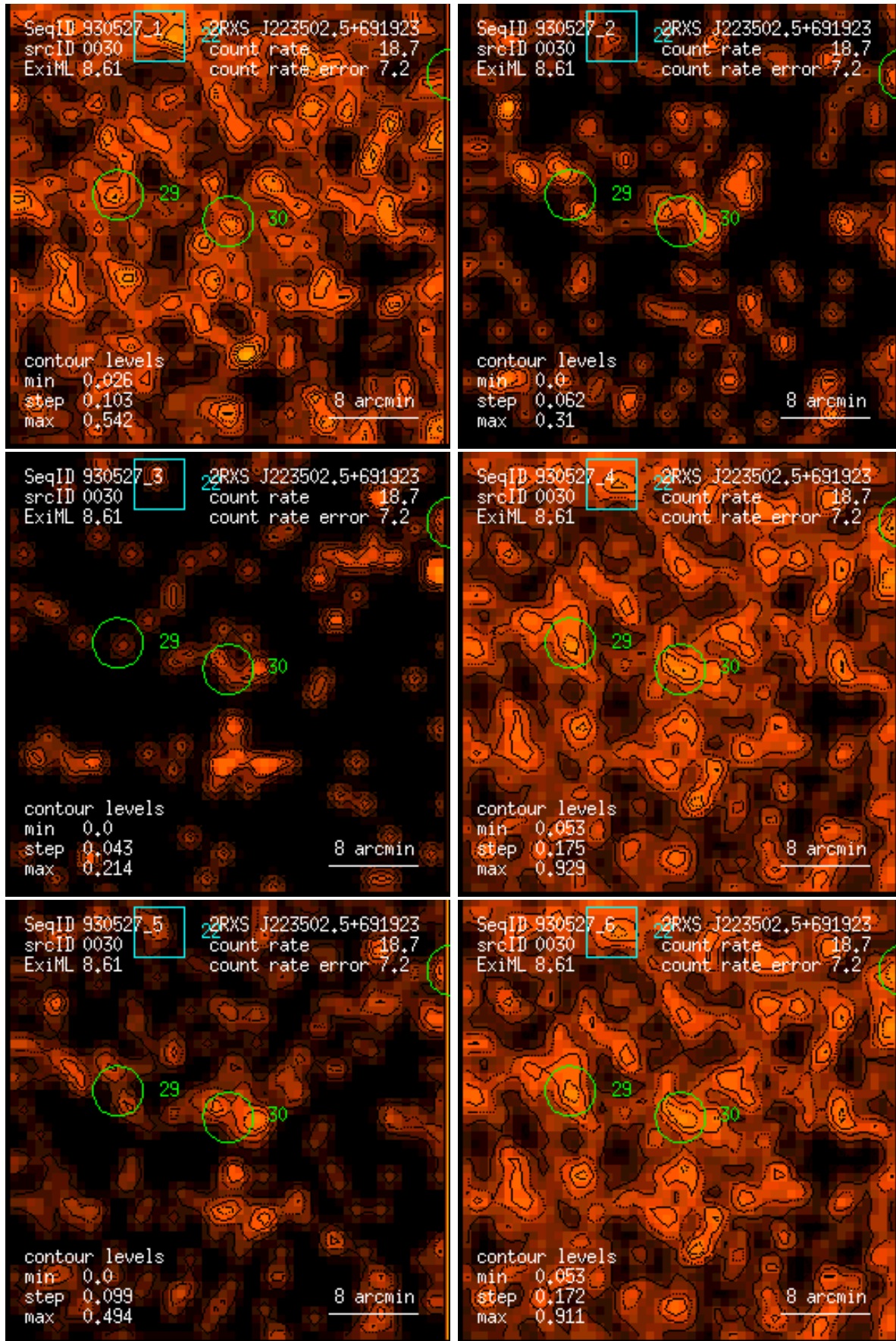
Figure 30: RASS 930527: detection 0030: band rate images, Gaussian filter: (1) PSPC channels 11 – 41, (2) 52 – 90, (3) 91 – 201, (4) 11 – 235, (5) 52 – 201, (6) 11 – 201. Broad band rates in counts/ks. Band rate contour levels in counts/ks/arcmin 2 .
