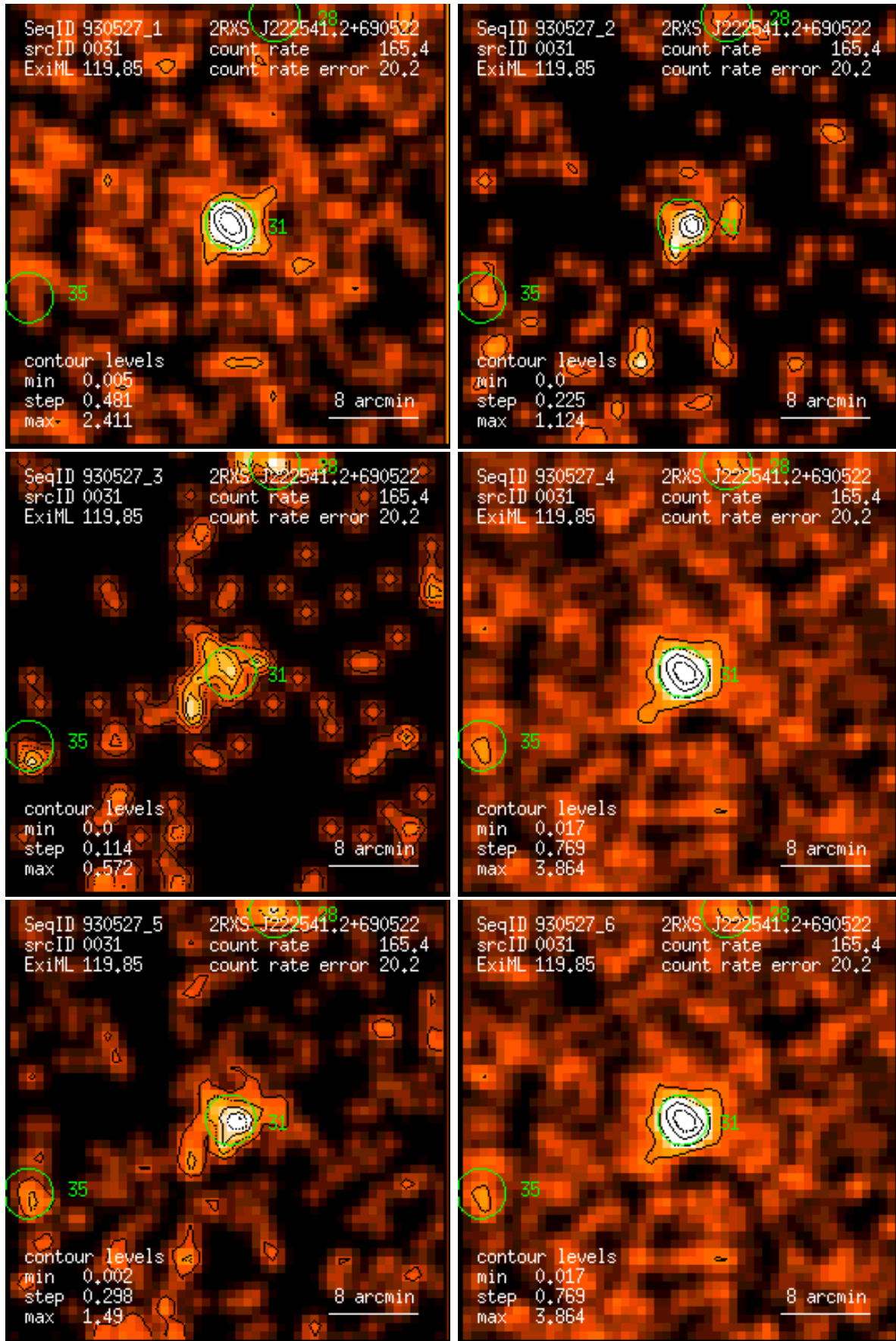
Figure 31: RASS 930527: detection 0031: band rate images, Gaussian filter: (1) PSPC channels 11 – 41, (2) 52 – 90, (3) 91 – 201, (4) 11 – 235, (5) 52 – 201, (6) 11 – 201. Broad band rates in counts/ks. Band rate contour levels in counts/ks/arcmin 2 .
