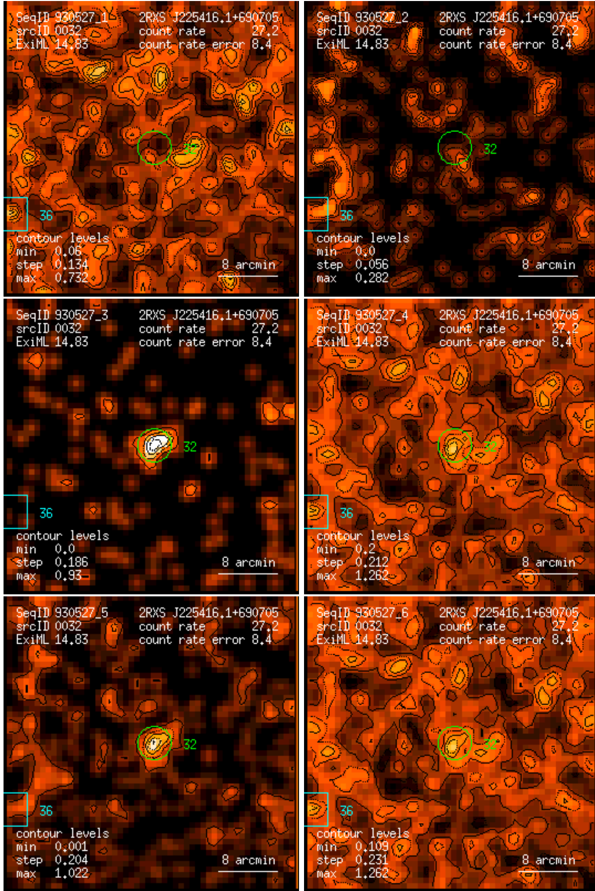
Figure 32: RASS 930527: detection 0032: band rate images, Gaussian filter: (1) PSPC channels 11 – 41, (2) 52 – 90, (3) 91 – 201, (4) 11 – 235, (5) 52 – 201, (6) 11 – 201. Broad band rates in counts/ks. Band rate contour levels in counts/ks/arcmin 2 .
