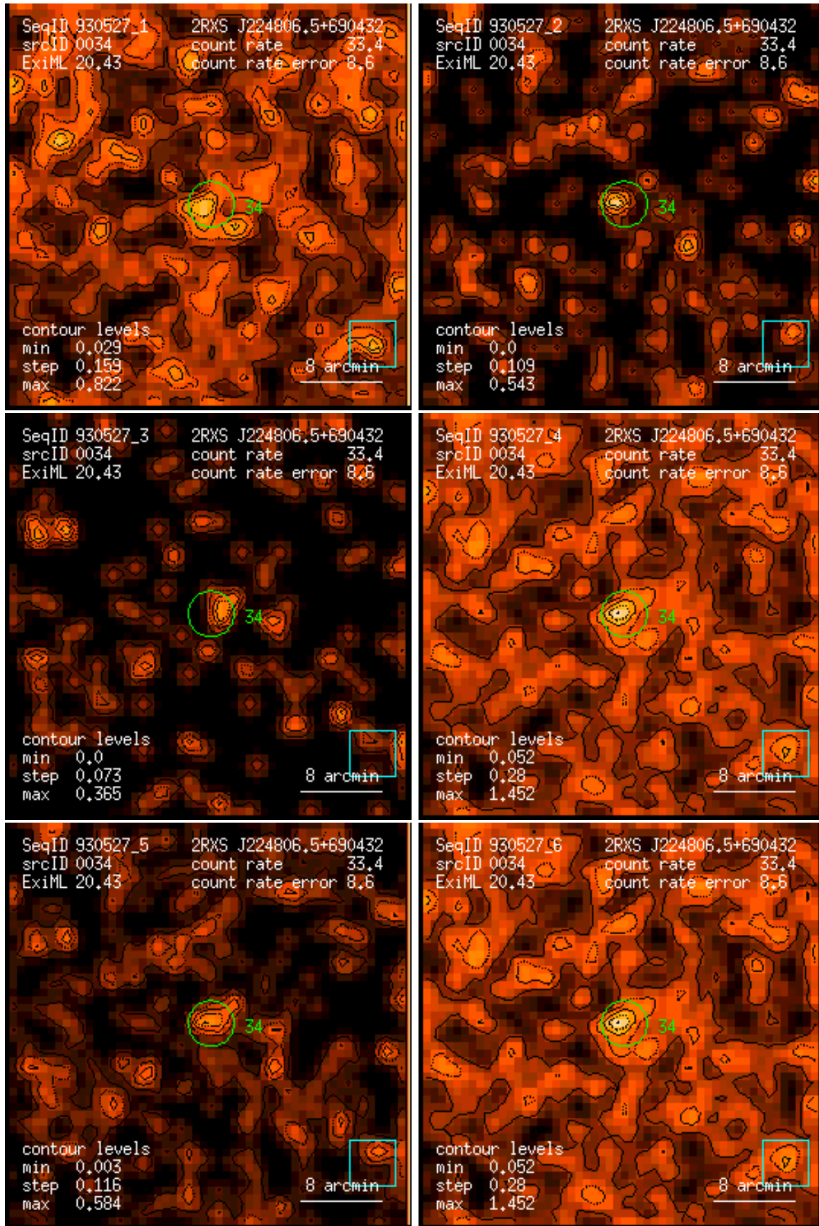
Figure 34: RASS 930527: detection 0034: band rate images, Gaussian filter: (1) PSPC channels 11 – 41, (2) 52 – 90, (3) 91 – 201, (4) 11 – 235, (5) 52 – 201, (6) 11 – 201. Broad band rates in counts/ks. Band rate contour levels in counts/ks/arcmin 2 .
