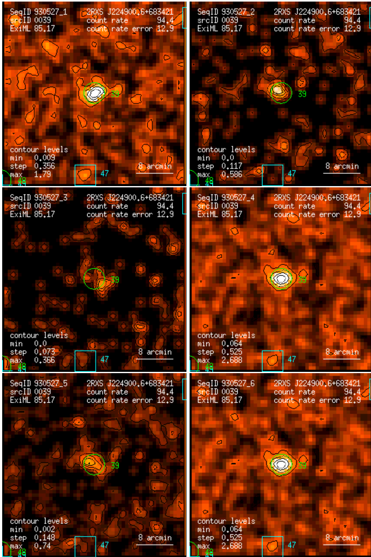
Figure 39: RASS 930527: detection 0039: band rate images, Gaussian filter: (1) PSPC channels 11 – 41, (2) 52 – 90, (3) 91 – 201, (4) 11 – 235, (5) 52 – 201, (6) 11 – 201. Broad band rates in counts/ks. Band rate contour levels in counts/ks/arcmin 2 .
