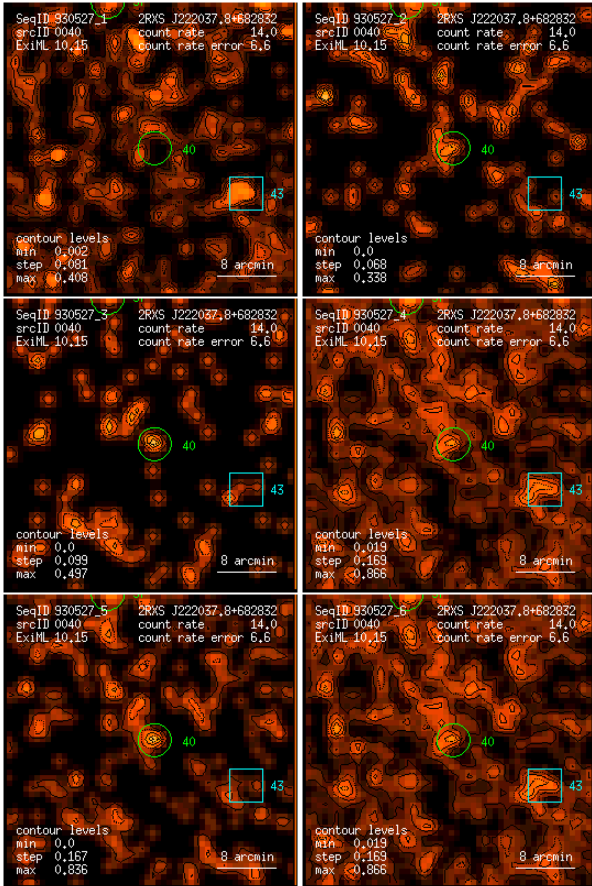
Figure 40: RASS 930527: detection 0040: band rate images, Gaussian filter: (1) PSPC channels 11 – 41, (2) 52 – 90, (3) 91 – 201, (4) 11 – 235, (5) 52 – 201, (6) 11 – 201. Broad band rates in counts/ks. Band rate contour levels in counts/ks/arcmin 2 .
