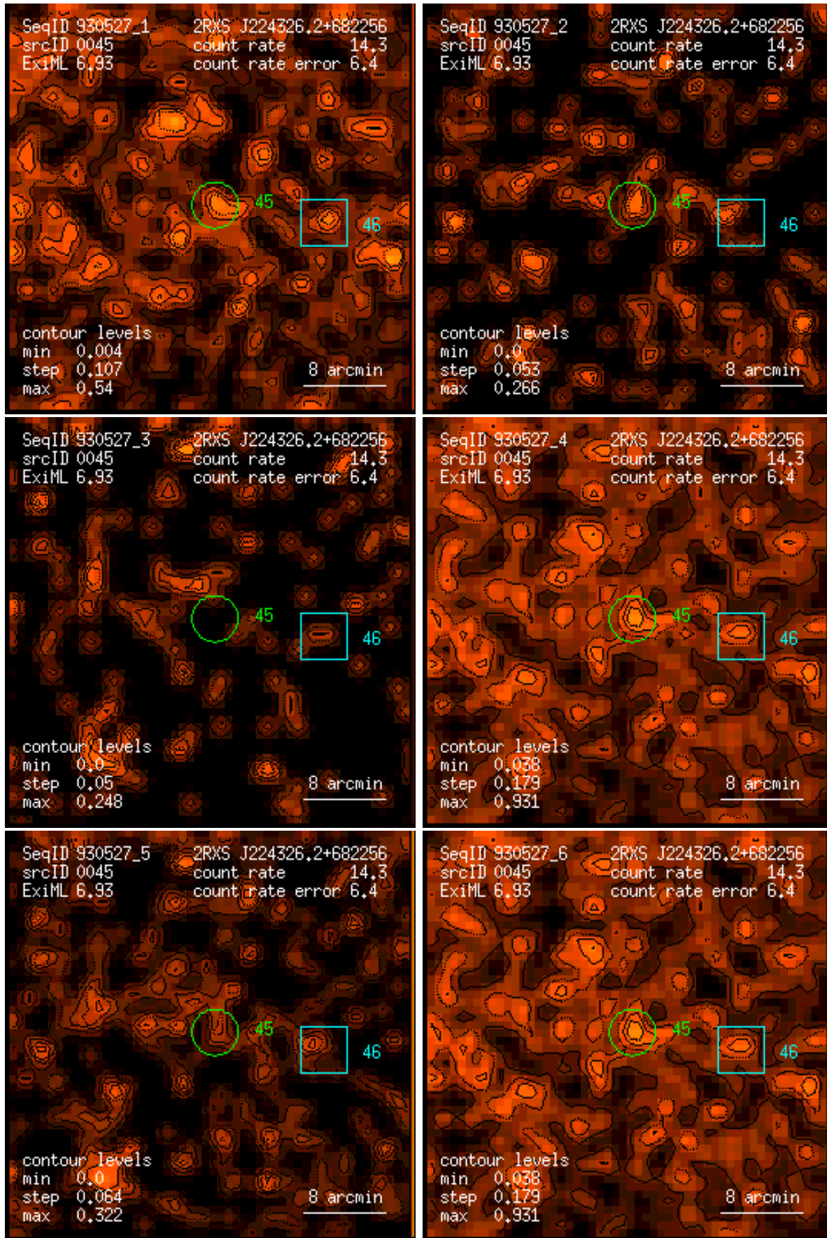
Figure 45: RASS 930527: detection 0045: band rate images, Gaussian filter: (1) PSPC channels 11 – 41, (2) 52 – 90, (3) 91 – 201, (4) 11 – 235, (5) 52 – 201, (6) 11 – 201. Broad band rates in counts/ks. Band rate contour levels in counts/ks/arcmin 2 .
