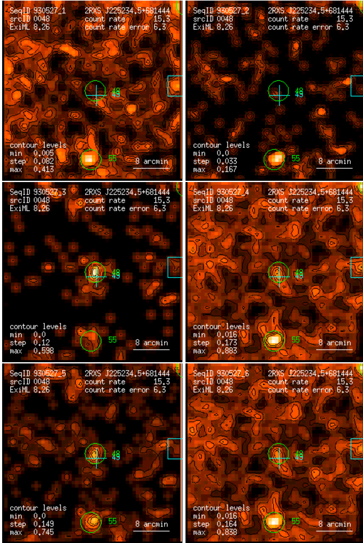
Figure 48: RASS 930527: detection 0048: band rate images, Gaussian filter: (1) PSPC channels 11 – 41, (2) 52 – 90, (3) 91 – 201, (4) 11 – 235, (5) 52 – 201, (6) 11 – 201. Broad band rates in counts/ks. Band rate contour levels in counts/ks/arcmin 2 .
