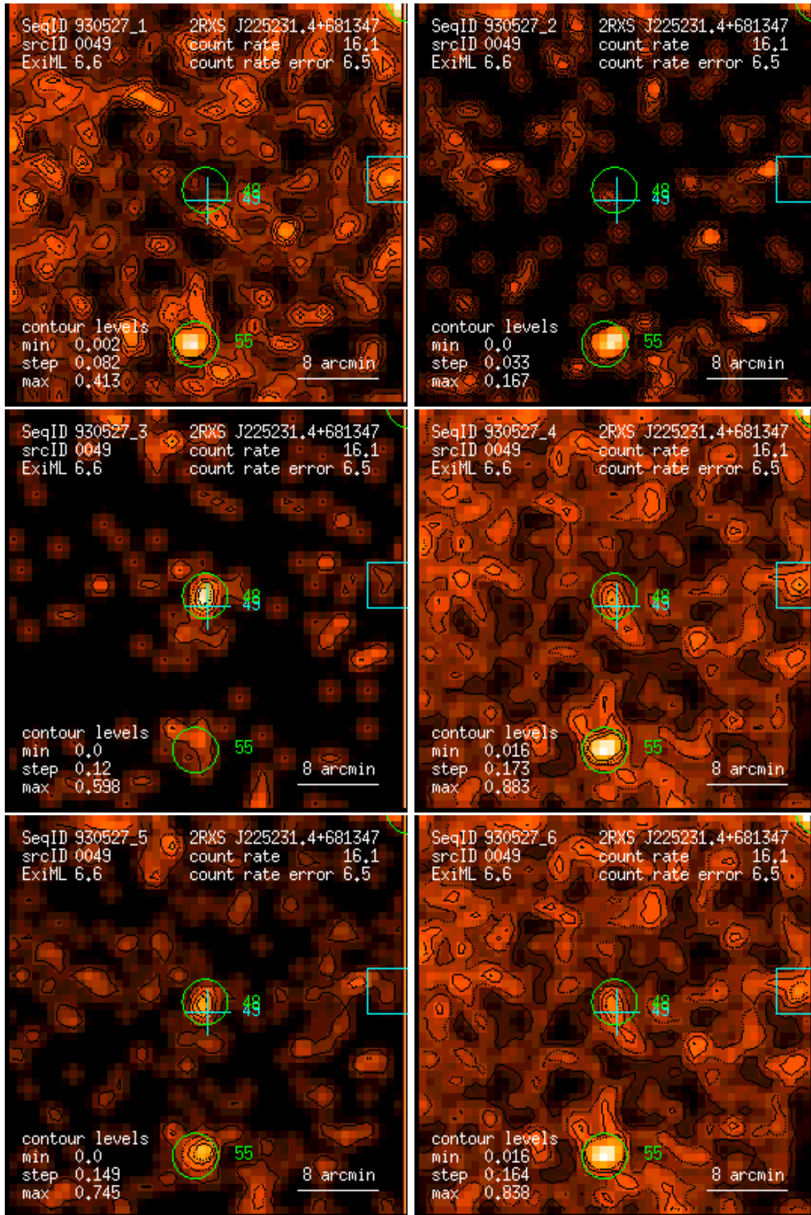
Figure 49: RASS 930527: detection 0049: band rate images, Gaussian filter: (1) PSPC channels 11 – 41, (2) 52 – 90, (3) 91 – 201, (4) 11 – 235, (5) 52 – 201, (6) 11 – 201. Broad band rates in counts/ks. Band rate contour levels in counts/ks/arcmin 2 .
