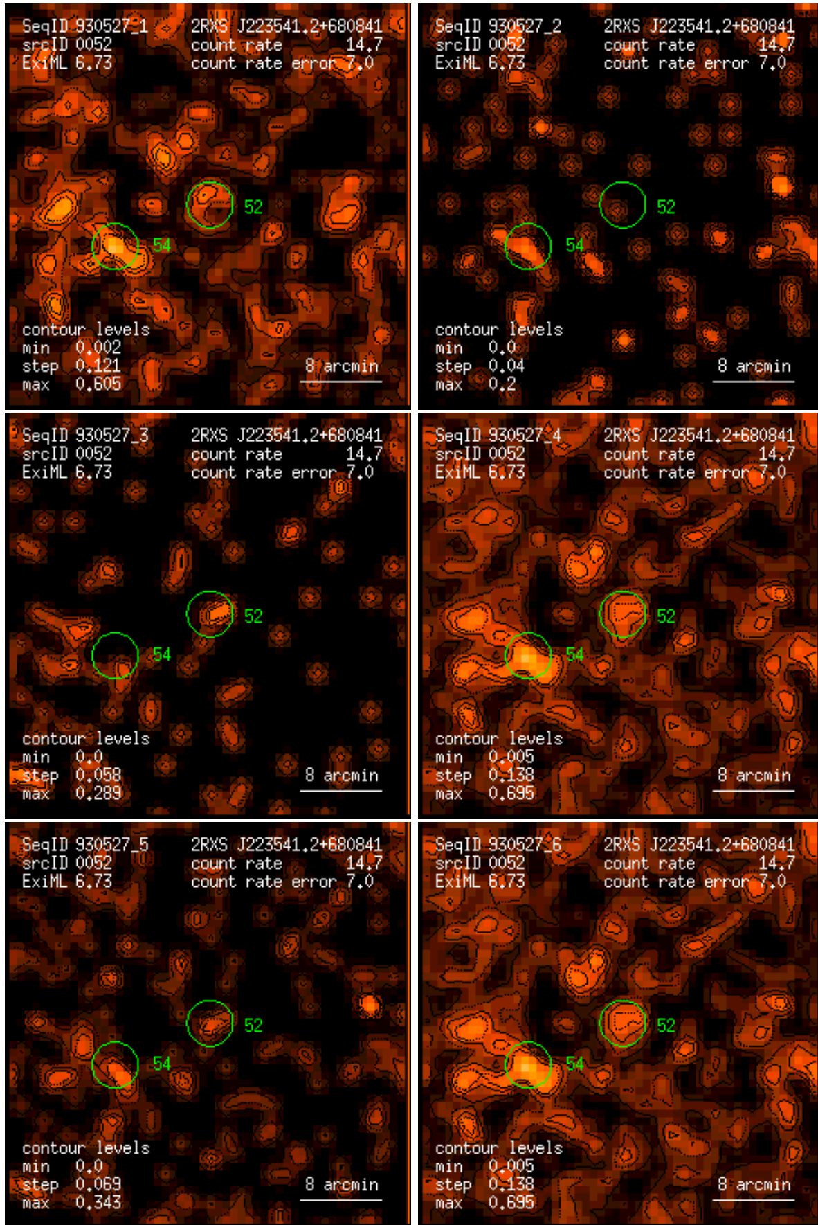
Figure 52: RASS 930527: detection 0052: band rate images, Gaussian filter: (1) PSPC channels 11 – 41, (2) 52 – 90, (3) 91 – 201, (4) 11 – 235, (5) 52 – 201, (6) 11 – 201. Broad band rates in counts/ks. Band rate contour levels in counts/ks/arcmin 2 .
