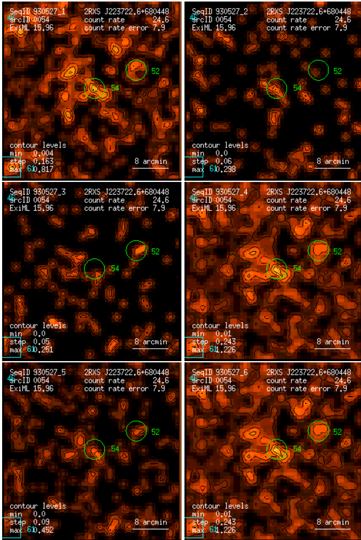
Figure 54: RASS 930527: detection 0054: band rate images, Gaussian filter: (1) PSPC channels 11 – 41, (2) 52 – 90, (3) 91 – 201, (4) 11 – 235, (5) 52 – 201, (6) 11 – 201. Broad band rates in counts/ks. Band rate contour levels in counts/ks/arcmin 2 .
