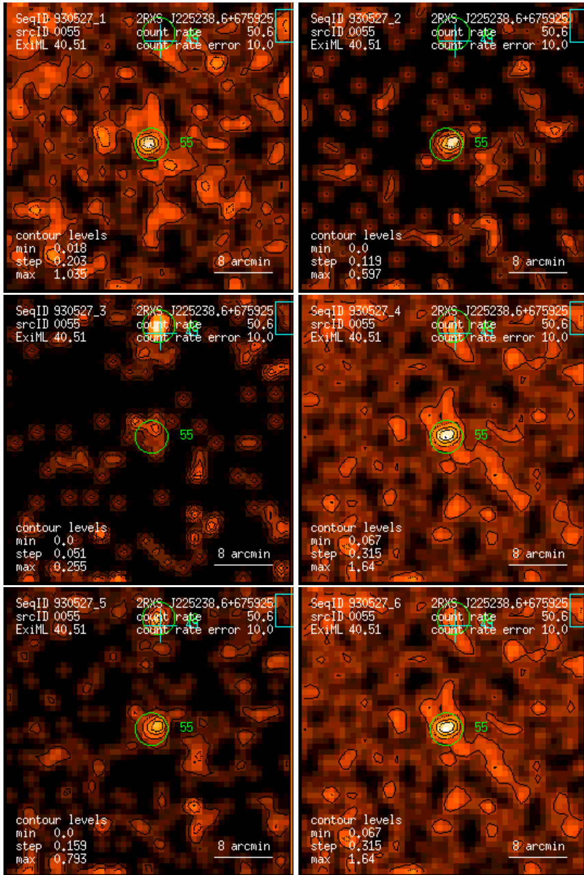
Figure 55: RASS 930527: detection 0055: band rate images, Gaussian filter: (1) PSPC channels 11 – 41, (2) 52 – 90, (3) 91 – 201, (4) 11 – 235, (5) 52 – 201, (6) 11 – 201. Broad band rates in counts/ks. Band rate contour levels in counts/ks/arcmin 2 .
