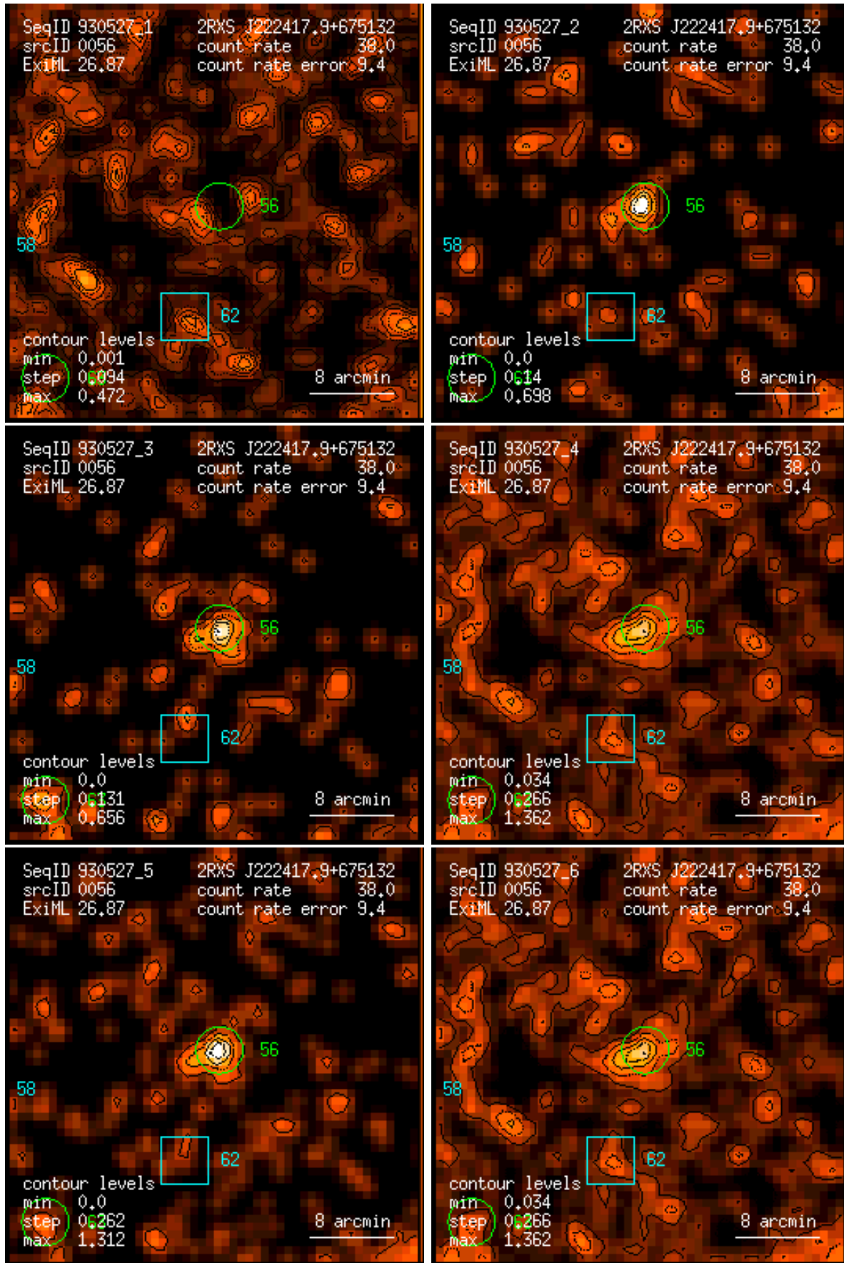
Figure 56: RASS 930527: detection 0056: band rate images, Gaussian filter: (1) PSPC channels 11 – 41, (2) 52 – 90, (3) 91 – 201, (4) 11 – 235, (5) 52 – 201, (6) 11 – 201. Broad band rates in counts/ks. Band rate contour levels in counts/ks/arcmin 2 .
