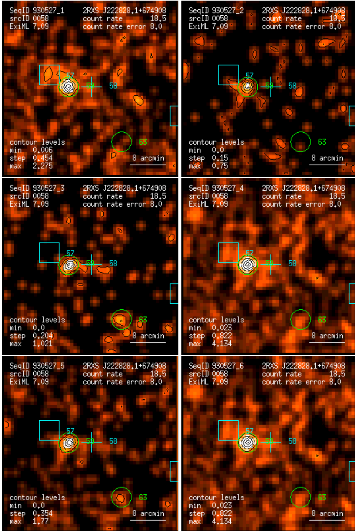
Figure 58: RASS 930527: detection 0058: band rate images, Gaussian filter: (1) PSPC channels 11 – 41, (2) 52 – 90, (3) 91 – 201, (4) 11 – 235, (5) 52 – 201, (6) 11 – 201. Broad band rates in counts/ks. Band rate contour levels in counts/ks/arcmin 2 .
