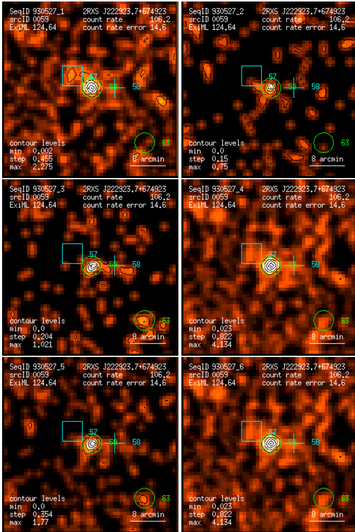
Figure 59: RASS 930527: detection 0059: band rate images, Gaussian filter: (1) PSPC channels 11 – 41, (2) 52 – 90, (3) 91 – 201, (4) 11 – 235, (5) 52 – 201, (6) 11 – 201. Broad band rates in counts/ks. Band rate contour levels in counts/ks/arcmin 2 .
